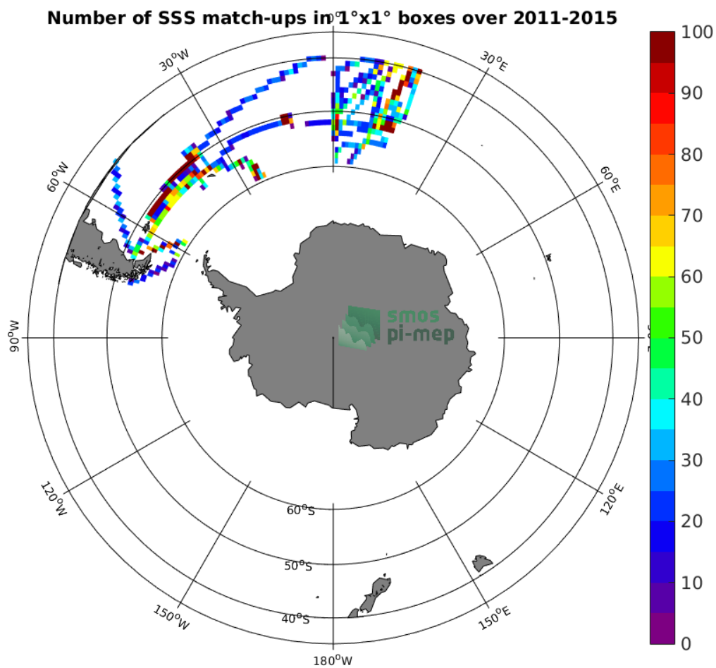
Figure 4: Number of SSS match-ups between TSG-POLARSTERN SSS and the Aquarius-L3-OR-V5-7DAY-RUNNING-RAIN-MASK-1DEG SSS product for the Roaring Forties and Furious Fifties Pi-MEP region over 1^\circ \times 1^\circ boxes and for the full satellite product period.
