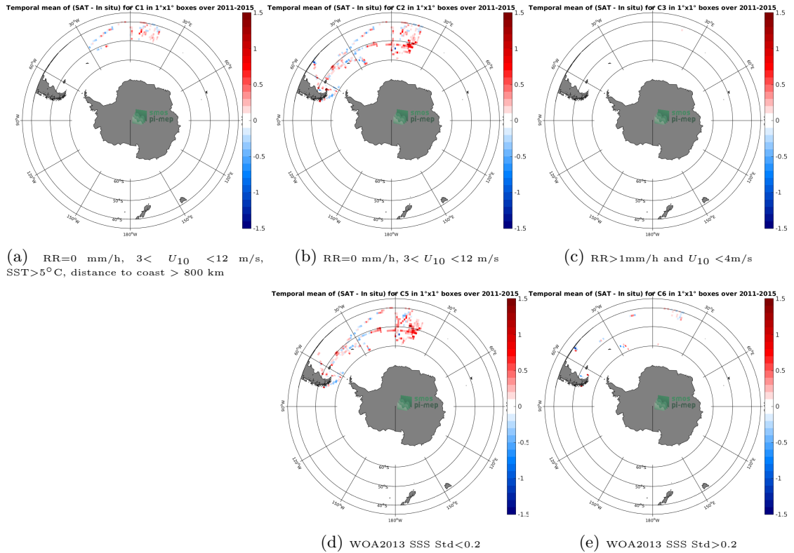
Figure 12: Temporal mean gridded over spatial boxes of size 1^\circ \times 1^\circ of \Delta SSS (Aquarius-L3-OR-V5-7DAY-RUNNING-RAIN-MASK-1DEG - TSG-POLARSTERN) for 5 different subdatasets corresponding to: RR=0 mm/h, 3 < U_{10} < 12 m/s, SST >5^\circ C, distance to coast > 800 km (a), RR=0 mm/h, 3 < U_{10} < 12 m/s (b), RR >1 mm/h and U_{10} < 4 m/s (c), WOA2013 SSS Std <0.2 (d), WOA2013 SSS Std >0.2 (e).
