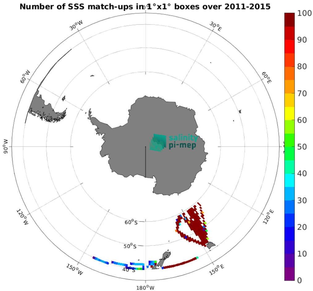
Figure 5: Number of SSS match-ups between TSG (LEGOS-DM) SSS and the Aquarius SSS L3 OR v5 - 7-Day running - Rain mask (NASA-GSFC) SSS product for the Roaring Forties and Furious Fifties Pi-MEP region over 1^\circ \times 1^\circ boxes and for the full satellite product period.
