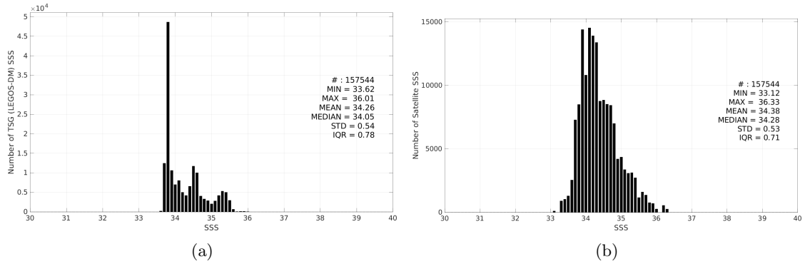
Figure 3: Histograms of SSS from TSG (LEGOS-DM) (a) and Aquarius SSS L3 OR v5 - 7-Day running - Rain mask (NASA-GSFC) (b) considering all match-up pairs per bins of 0.1 over the Roaring Forties and Furious Fifties Pi-MEP region and for the full satellite product period.
