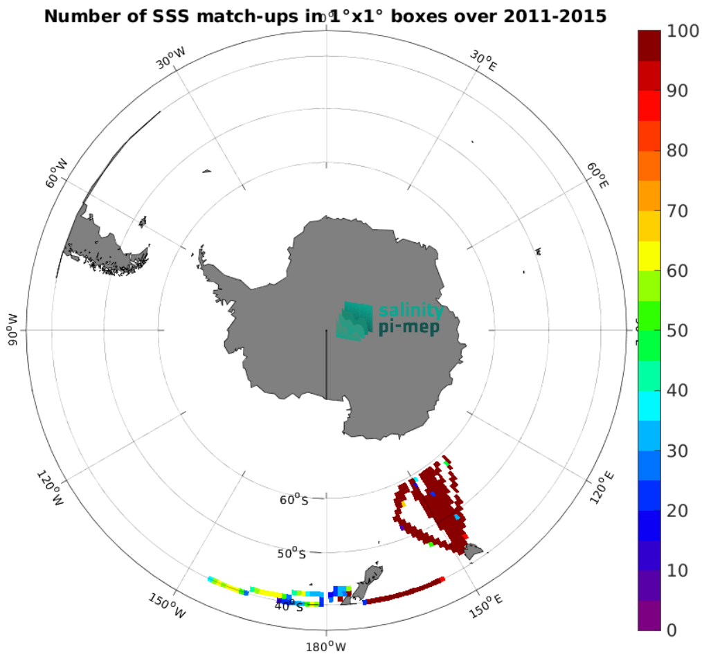
Figure 4: Number of SSS match-ups between TSG (LEGOS-DM) SSS and the Aquarius SSS L3 OR v5 - 7-Day running - Rain mask (NASA-GSFC) SSS product for the Roaring Forties and Furious Fifties Pi-MEP region over 1^\circ \times 1^\circ boxes and for the full satellite product period.
