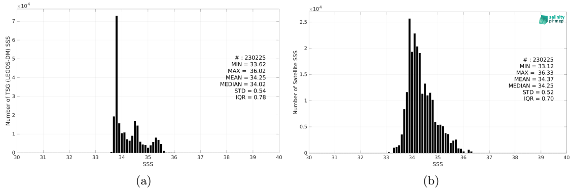
Figure 2: Histograms of SSS from TSG (LEGOS-DM) (a) and Aquarius SSS L3 OR v5 - 7-Day running - Rain mask (NASA-GSFC) (b) considering all match-up pairs per bins of 0.1 over the Roaring Forties and Furious Fifties Pi-MEP region and for the full satellite product period.
