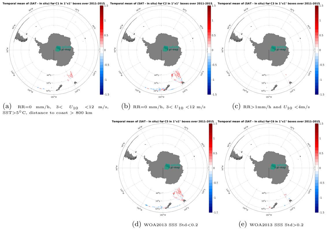
Figure 12: Temporal mean gridded over spatial boxes of size 1^{\circ}\times 1^{\circ} of \Delta\text{SSS} (Aquarius SSS L3 OR v5 - 7-Day running - Rain mask (NASA-GSFC) - TSG (LEGOS-DM)) for 5 different subdatasets corresponding to:RR=0 mm/h, 3 < U_{10} < 12 m/s, SST > 5^{\circ}\text{C} , distance to coast > 800 km (a), RR=0 mm/h, 3 < U_{10} < 12 m/s (b), RR > 1 mm/h and U_{10} < 4 m/s (c), WOA2013 SSS Std < 0.2 (d), WOA2013 SSS Std > 0.2 (e).
