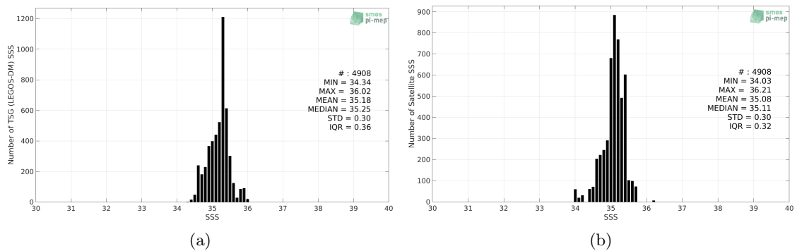
Figure 2: Histograms of SSS from TSG (LEGOS-DM) (a) and Aquarius SSS L3 OR v5 - 7-Day running - Rain mask (NASA-GSFC) (b) considering all match-up pairs per bins of 0.1 over the Roaring Forties and Furious Fifties Pi-MEP region and for the full satellite product period.
