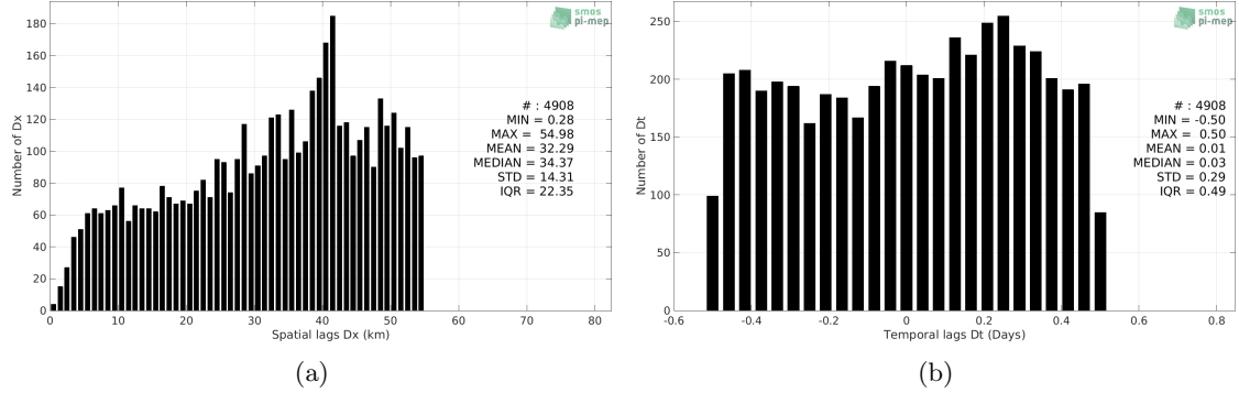
Figure 5: Histograms of the spatial (a) and temporal (b) lags between the time of the TSG (LEGOS-DM) measurements and the date of the corresponding Aquarius SSS L3 OR v5 - 7-Day running - Rain mask (NASA-GSFC) SSS product.
