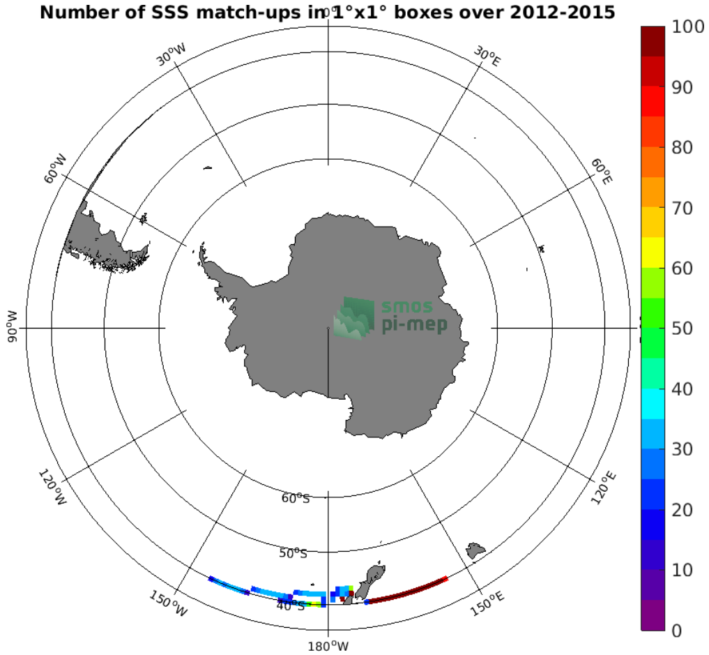
Figure 4: Number of SSS match-ups between TSG (LEGOS-DM) SSS and the Aquarius SSS L3 OR v5 - 7-Day running - Rain mask (NASA-GSFC) SSS product for the Roaring Forties and Furious Fifties Pi-MEP region over 1°x1° boxes and for the full satellite product period.
