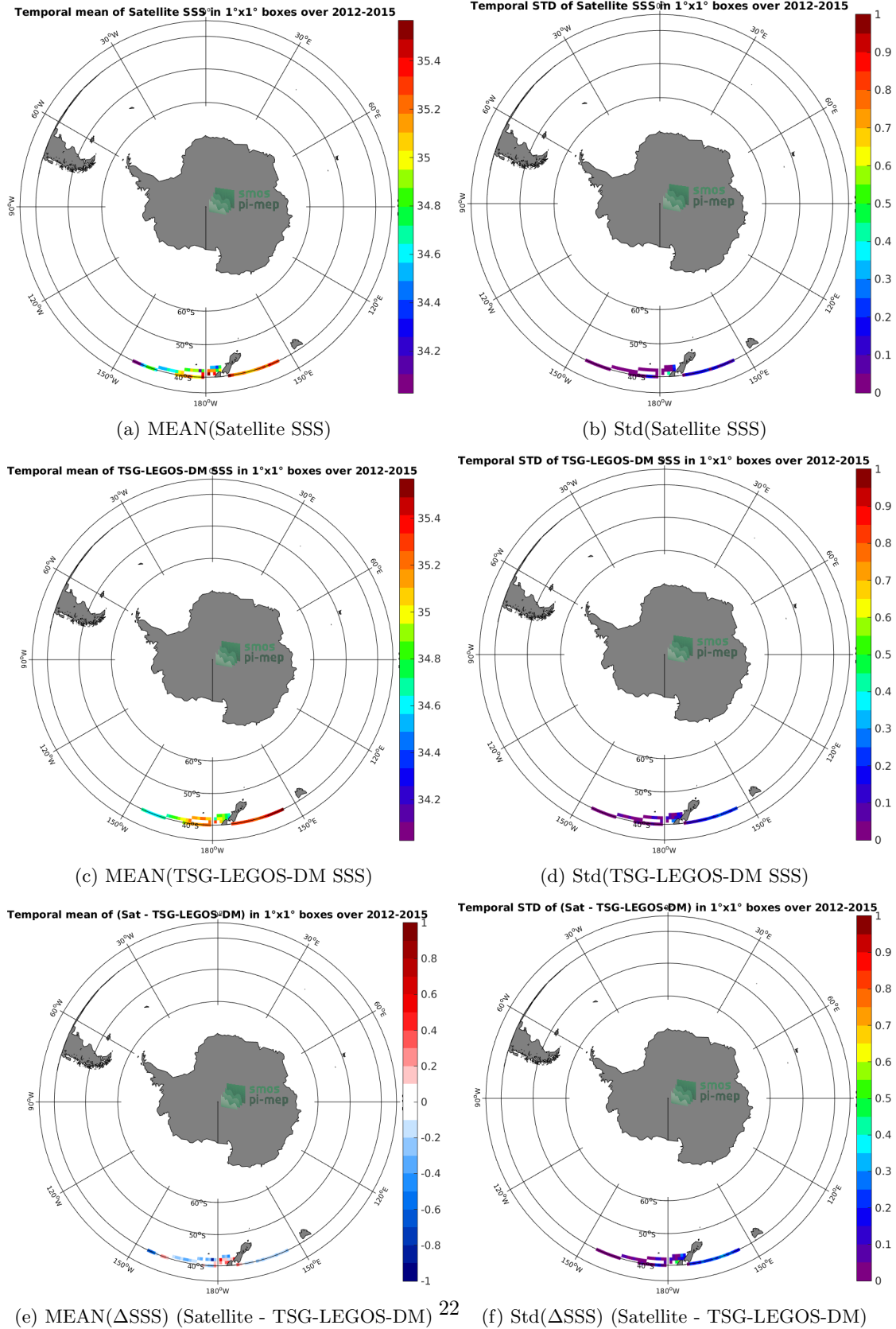
Figure 6: Temporal mean (left) and Std (right) of SSS from Aquarius-L3-OR-V5-7DAY-RUNNING-RAIN-MASK-1DEG (top), TSG-LEGOS-DM (middle), and of \Delta SSS (Satellite - TSG-LEGOS-DM). Only match-up pairs are used to generate these maps.
