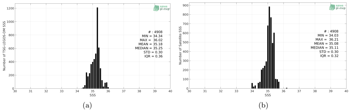
Figure 2: Histograms of SSS from TSG-LEGOS-DM (a) and Aquarius-L3-OR-V5-7DAY-RUNNING-RAIN-MASK-1DEG (b) considering all match-up pairs per bins of 0.1 over the Roaring Forties and Furious Fifties Pi-MEP region and for the full satellite product period.
