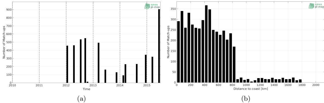
Figure 1: Number of match-ups between TSG-LEGOS-DM and Aquarius-L3-OR-V5-7DAY-RUNNING-RAIN-MASK-1DEG SSS as a function of time (a) and as function of the distance to coast (b) over the Roaring Forties and Furious Fifties Pi-MEP region and for the full satellite product period.
