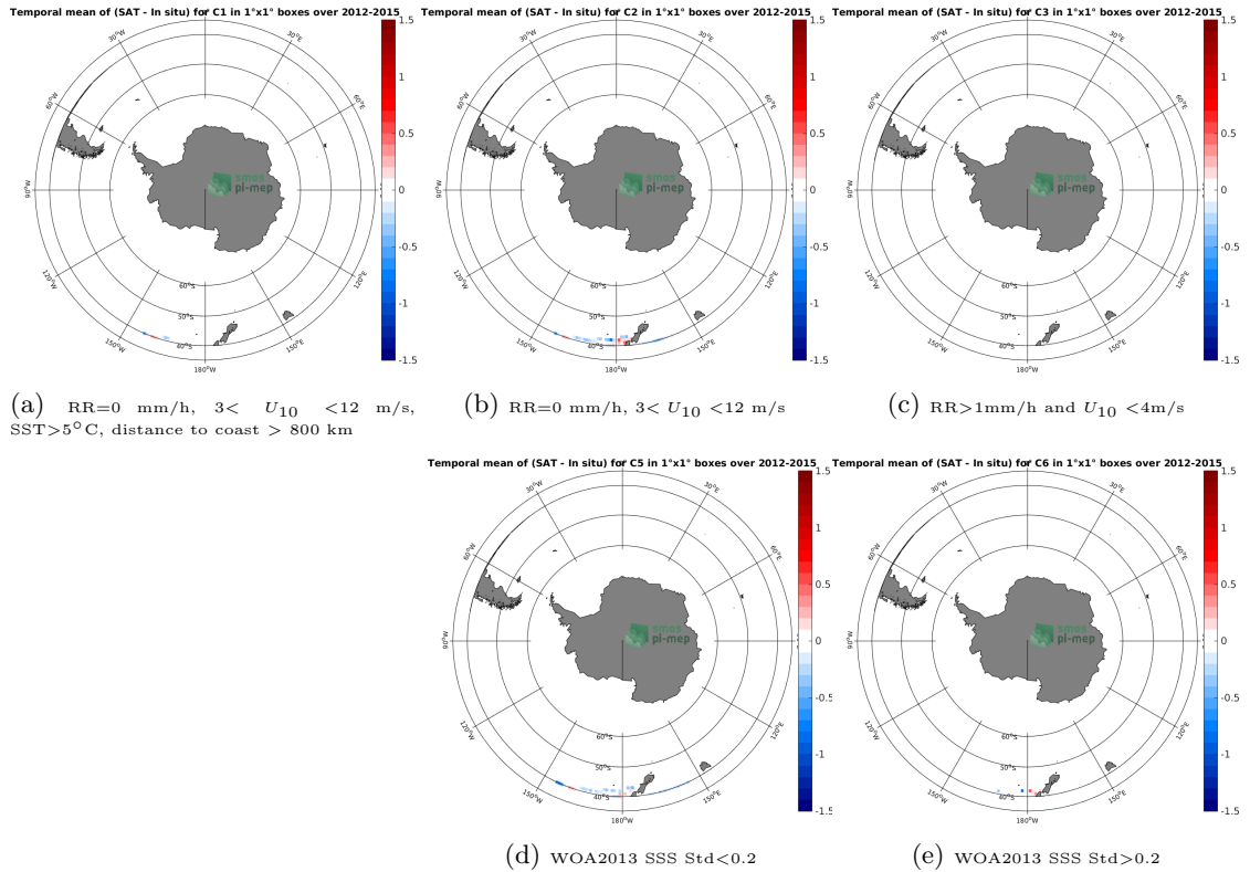
Figure 12: Temporal mean gridded over spatial boxes of size 1^\circ \times 1^\circ of \Delta SSS (Aquarius-L3-OR-V5-7DAY-RUNNING-RAIN-MASK-1DEG - TSG-LEGOS-DM) for 5 different subdatasets corresponding to: RR=0 mm/h, 3 < U_{10} < 12 m/s, SST > 5^\circ\text{C} , distance to coast > 800 km (a), RR=0 mm/h, 3 < U_{10} < 12 m/s (b), RR > 1 mm/h and U_{10} < 4 m/s (c), WOA2013 SSS Std < 0.2 (d), WOA2013 SSS Std > 0.2 (e).
