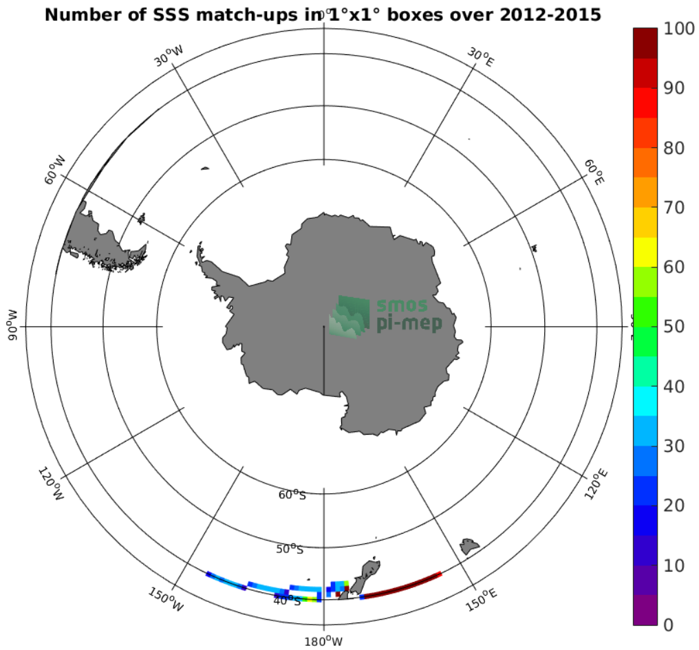
Figure 4: Number of SSS match-ups between TSG-LEGOS-DM SSS and the Aquarius-L3-OR-V5-7DAY-RUNNING-RAIN-MASK-1DEG SSS product for the Roaring Forties and Furious Fifties Pi-MEP region over 1°x1° boxes and for the full satellite product period.
