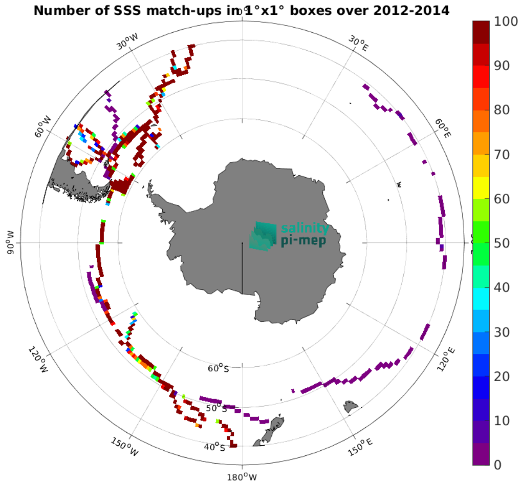
Figure 5: Number of SSS match-ups between TSG (GOSUD-Sailing-ship) SSS and the Aquarius SSS L3 OR v5 - 7-Day running - Rain mask (NASA-GSFC) SSS product for the Roaring Forties and Furious Fifties Pi-MEP region over 1^\circ \times 1^\circ boxes and for the full satellite product period.
