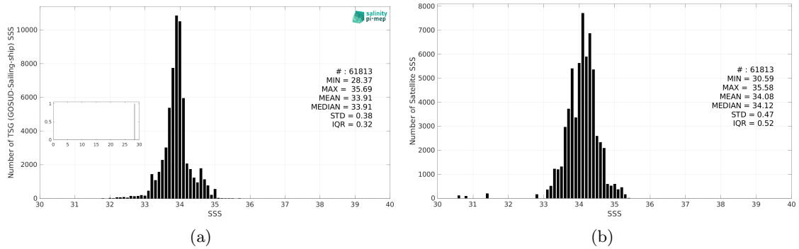
Figure 3: Histograms of SSS from TSG (GOSUD-Sailing-ship) (a) and Aquarius SSS L3 OR v5 - 7-Day running - Rain mask (NASA-GSFC) (b) considering all match-up pairs per bins of 0.1 over the Roaring Forties and Furious Fifties Pi-MEP region and for the full satellite product period.
