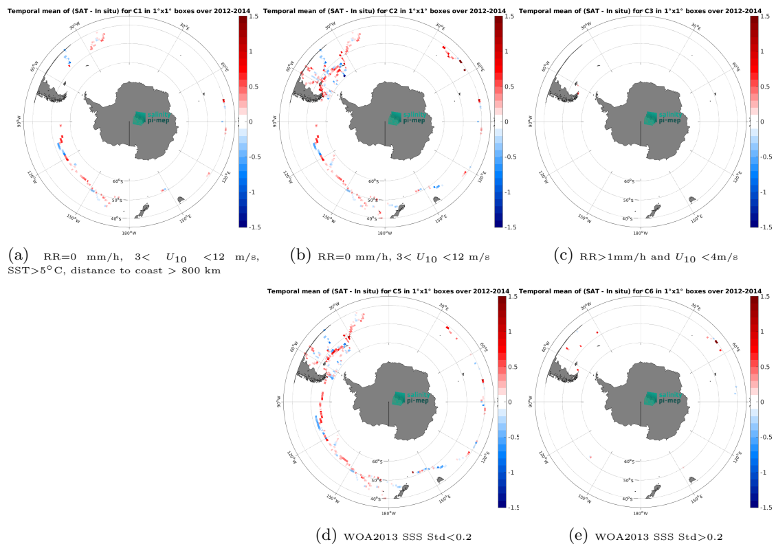
Figure 14: Temporal mean gridded over spatial boxes of size 1^\circ \times 1^\circ of \Delta\text{SSS} (Aquarius SSS L3 OR v5 - 7-Day running - Rain mask (NASA-GSFC) - TSG (GOSUD-Sailing-ship)) for 5 different subdatasets corresponding to:RR=0 mm/h, 3 < U_{10} < 12 m/s, SST>5°C, distance to coast > 800 km (a), RR=0 mm/h, 3 < U_{10} < 12 m/s (b), RR>1mm/h and U_{10} < 4 m/s (c), WOA2013 SSS Std<0.2 (d), WOA2013 SSS Std>0.2 (e).
