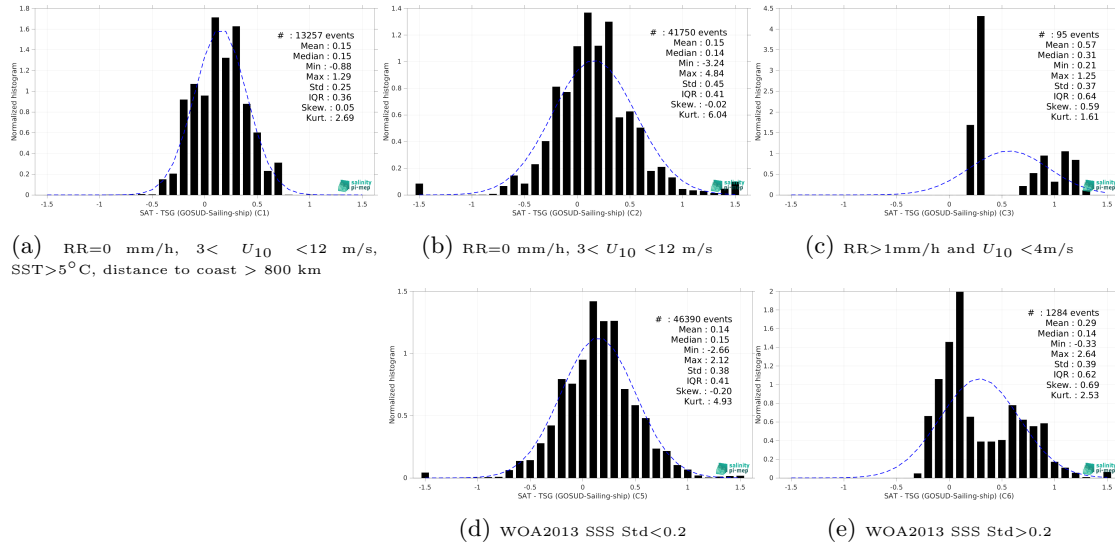
Figure 15: Normalized histogram of \Delta\text{SSS} (Aquarius SSS L3 OR v5 - 7-Day running - Rain mask (NASA-GSFC) - TSG (GOSUD-Sailing-ship)) for 5 different subdatasets corresponding to: RR=0 mm/h, 3 < U_{10} < 12 m/s, SST>5°C, distance to coast > 800 km (a), RR=0 mm/h, 3 < U_{10} < 12 m/s (b), RR>1mm/h and U_{10} < 4 m/s (c), WOA2013 SSS Std<0.2 (d), WOA2013 SSS Std>0.2 (e).
