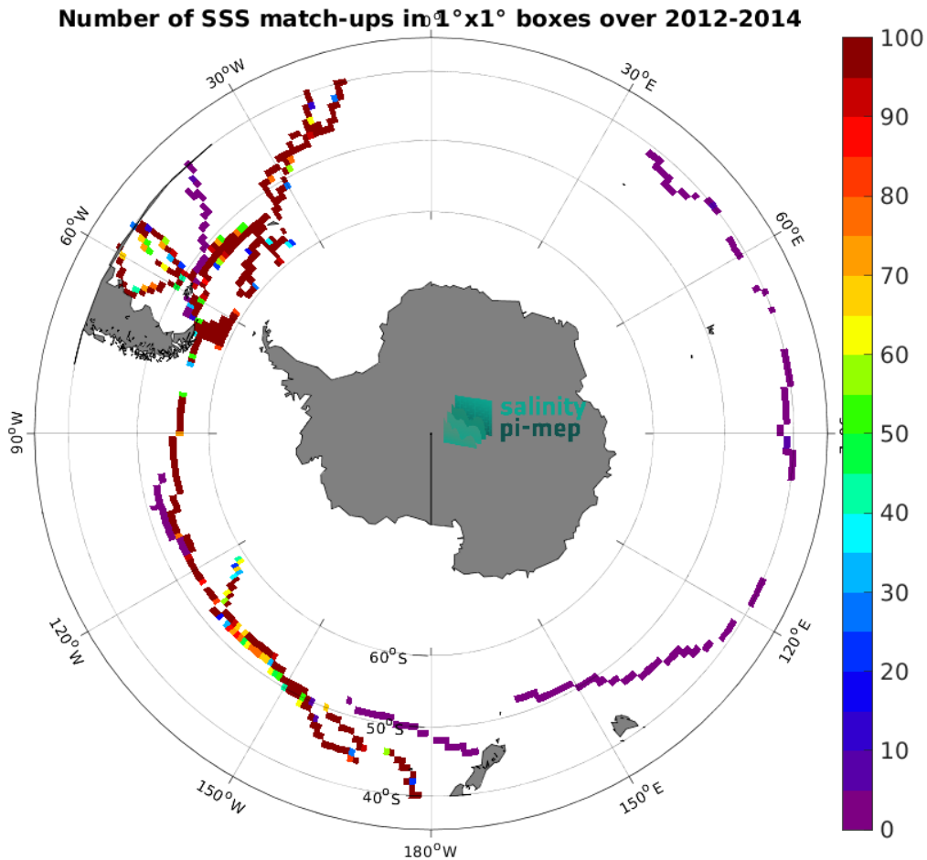
Figure 4: Number of SSS match-ups between TSG (GOSUD-Sailing-ship) SSS and the Aquarius SSS L3 OR v5 - 7-Day running - Rain mask (NASA-GSFC) SSS product for the Roaring Forties and Furious Fifties Pi-MEP region over 1^\circ \times 1^\circ boxes and for the full satellite product period.
