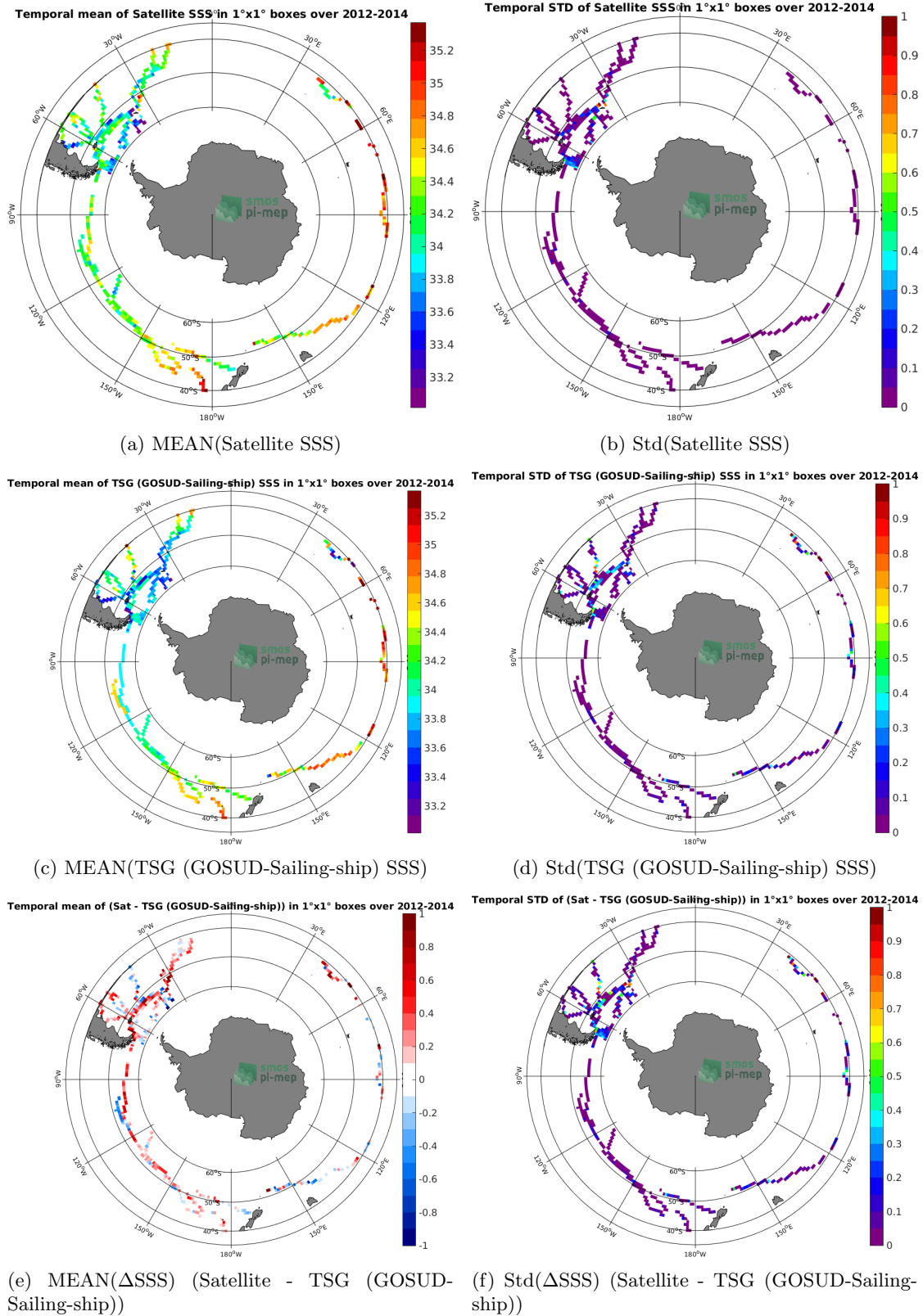
Figure 6: Temporal mean (left) and Std (right), of SSS from Aquarius SSS L3 OR v5 - 7-Day running - Rain mask (NASA-GSFC) (top), TSG (GOSUD-Sailing-ship) (middle), and of \Delta SSS (Satellite - TSG (GOSUD-Sailing-ship)). Only match-up pairs are used to generate these maps.
