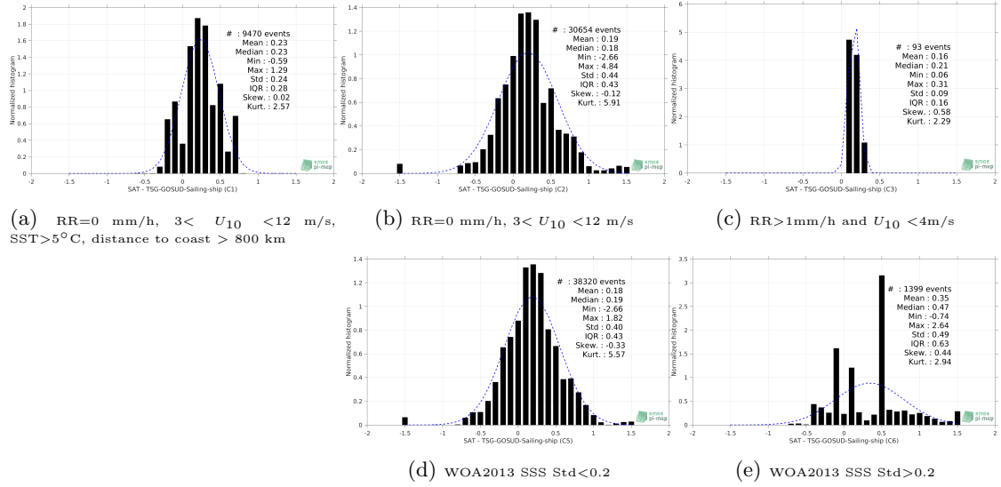
Figure 13: Normalized histogram of \Delta\text{SSS} (Aquarius-L3-OR-V5-7DAY-RUNNING-RAIN-MASK-1DEG - TSG-GOSUD-Sailing-ship) for 5 different subdatasets corresponding to: RR=0 mm/h, 3 < U_{10} < 12 m/s, SST > 5^\circ\text{C} , distance to coast > 800 km (a), RR=0 mm/h, 3 < U_{10} < 12 m/s (b), RR > 1\text{mm/h} and U_{10} < 4\text{m/s} (c), WOA2013 SSS Std < 0.2 (d), WOA2013 SSS Std > 0.2 (e).
