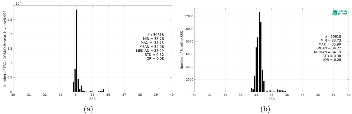
Figure 2: Histograms of SSS from TSG (GOSUD-Research-vessel) (a) and Aquarius SSS L3 OR v5 - 7-Day running - Rain mask (NASA-GSFC) (b) considering all match-up pairs per bins of 0.1 over the Roaring Forties and Furious Fifties Pi-MEP region and for the full satellite product period.
