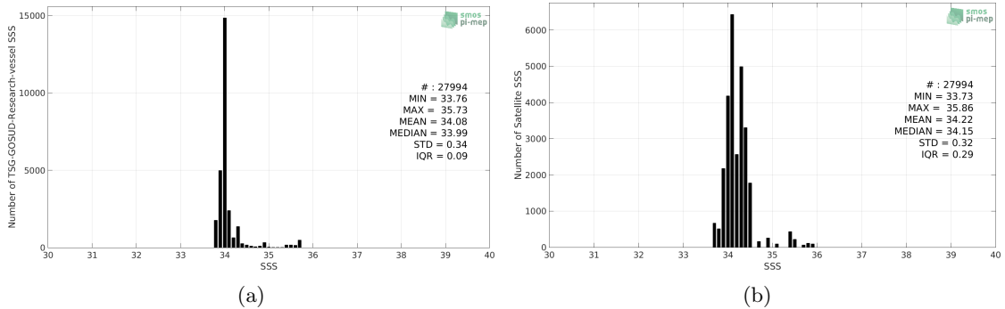
Figure 2: Histograms of SSS from TSG-GOSUD-Research-vessel (a) and Aquarius-L3-OR-V5-7DAY-RUNNING-RAIN-MASK-1DEG (b) considering all match-up pairs per bins of 0.1 over the Roaring Forties and Furious Fifties Pi-MEP region and for the full satellite product period.
