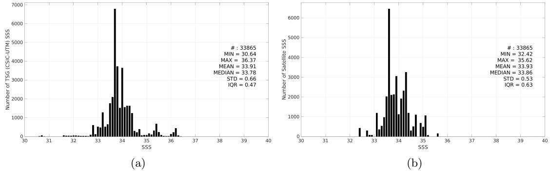
Figure 3: Histograms of SSS from TSG (CSIC-UTM) (a) and Aquarius SSS L3 OR v5 - 7-Day running - Rain mask (NASA-GSFC) (b) considering all match-up pairs per bins of 0.1 over the Roaring Forties and Furious Fifties Pi-MEP region and for the full satellite product period.
