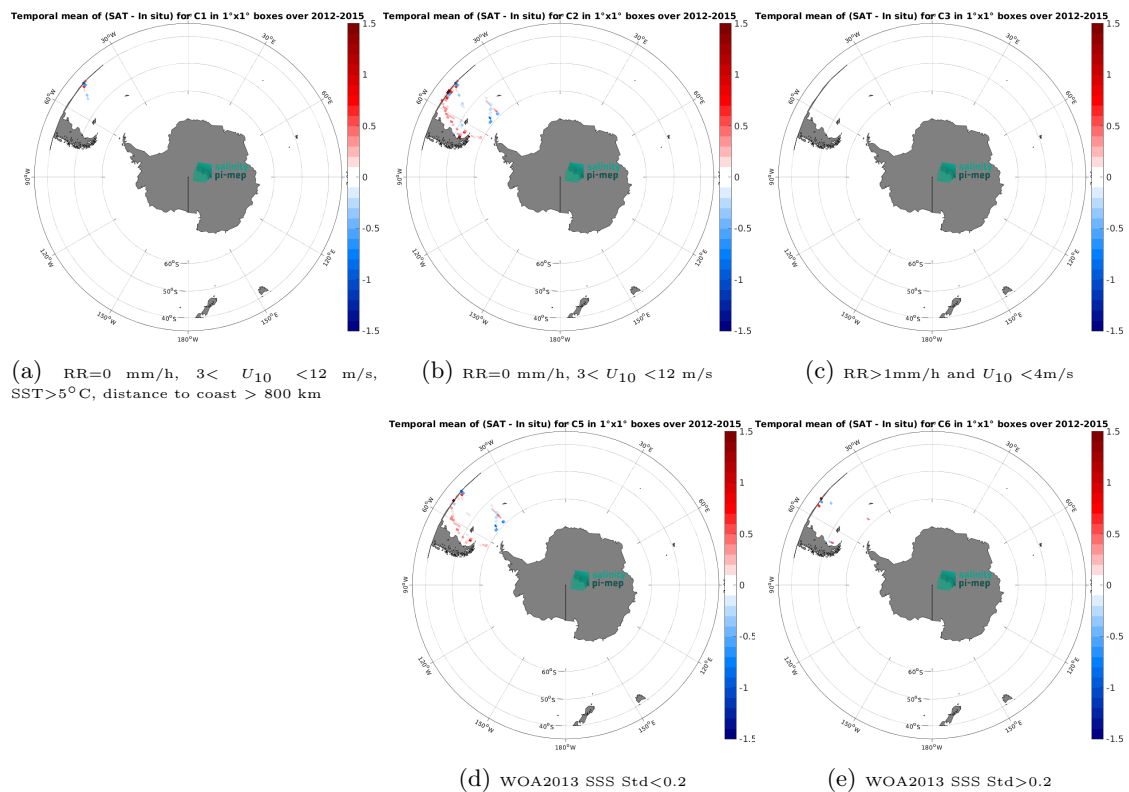
Figure 14: Temporal mean gridded over spatial boxes of size 1^\circ \times 1^\circ of \Delta\text{SSS} (Aquarius SSS L3 OR v5 - 7-Day running - Rain mask (NASA-GSFC) - TSG (CSIC-UTM)) for 5 different subdatasets corresponding to:RR=0 mm/h, 3 < U_{10} < 12 m/s, SST>5°C, distance to coast > 800 km (a), RR=0 mm/h, 3 < U_{10} < 12 m/s (b), RR>1mm/h and U_{10} < 4 m/s (c), WOA2013 SSS Std<0.2 (d), WOA2013 SSS Std>0.2 (e).
