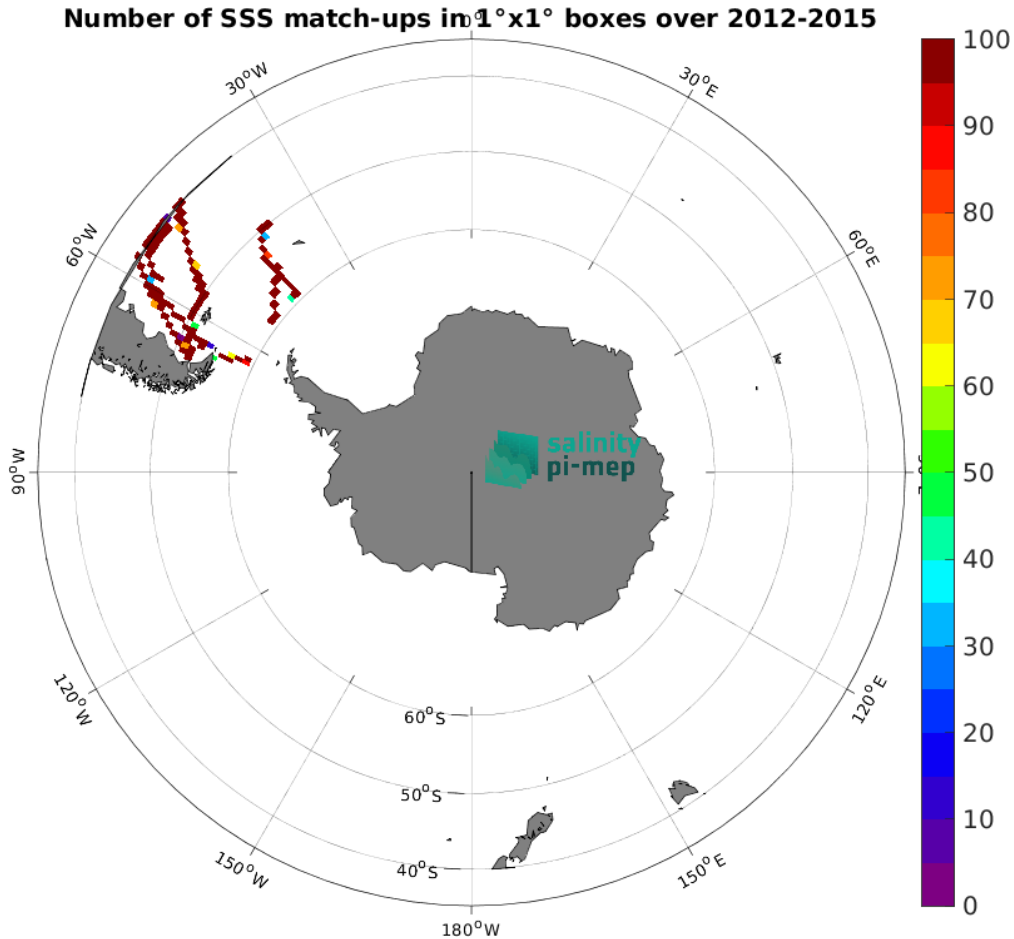
Figure 5: Number of SSS match-ups between TSG (CSIC-UTM) SSS and the Aquarius SSS L3 OR v5 - 7-Day running - Rain mask (NASA-GSFC) SSS product for the Roaring Forties and Furious Fifties Pi-MEP region over 1^\circ \times 1^\circ boxes and for the full satellite product period.
