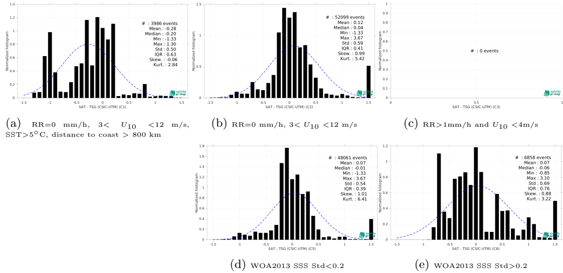
Figure 13: Normalized histogram of \Delta\text{SSS} (Aquarius SSS L3 OR v5 - 7-Day running - Rain mask (NASA-GSFC) - TSG (CSIC-UTM)) for 5 different subdatasets corresponding to: RR=0 mm/h, 3 < U_{10} < 12 m/s, SST>5°C, distance to coast > 800 km (a), RR=0 mm/h, 3 < U_{10} < 12 m/s (b), RR>1mm/h and U_{10} < 4 m/s (c), WOA2013 SSS Std<0.2 (d), WOA2013 SSS Std>0.2 (e).
