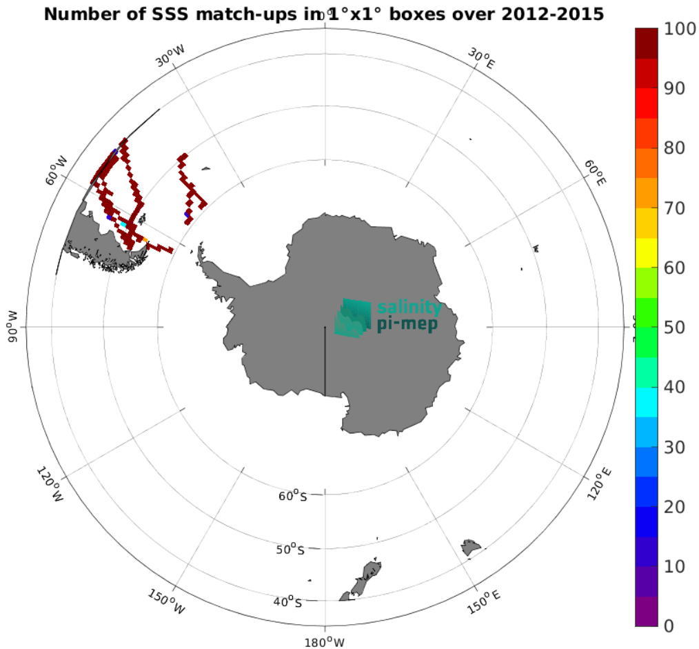
Figure 4: Number of SSS match-ups between TSG (CSIC-UTM) SSS and the Aquarius SSS L3 OR v5 - 7-Day running - Rain mask (NASA-GSFC) SSS product for the Roaring Forties and Furious Fifties Pi-MEP region over 1^\circ \times 1^\circ boxes and for the full satellite product period.
