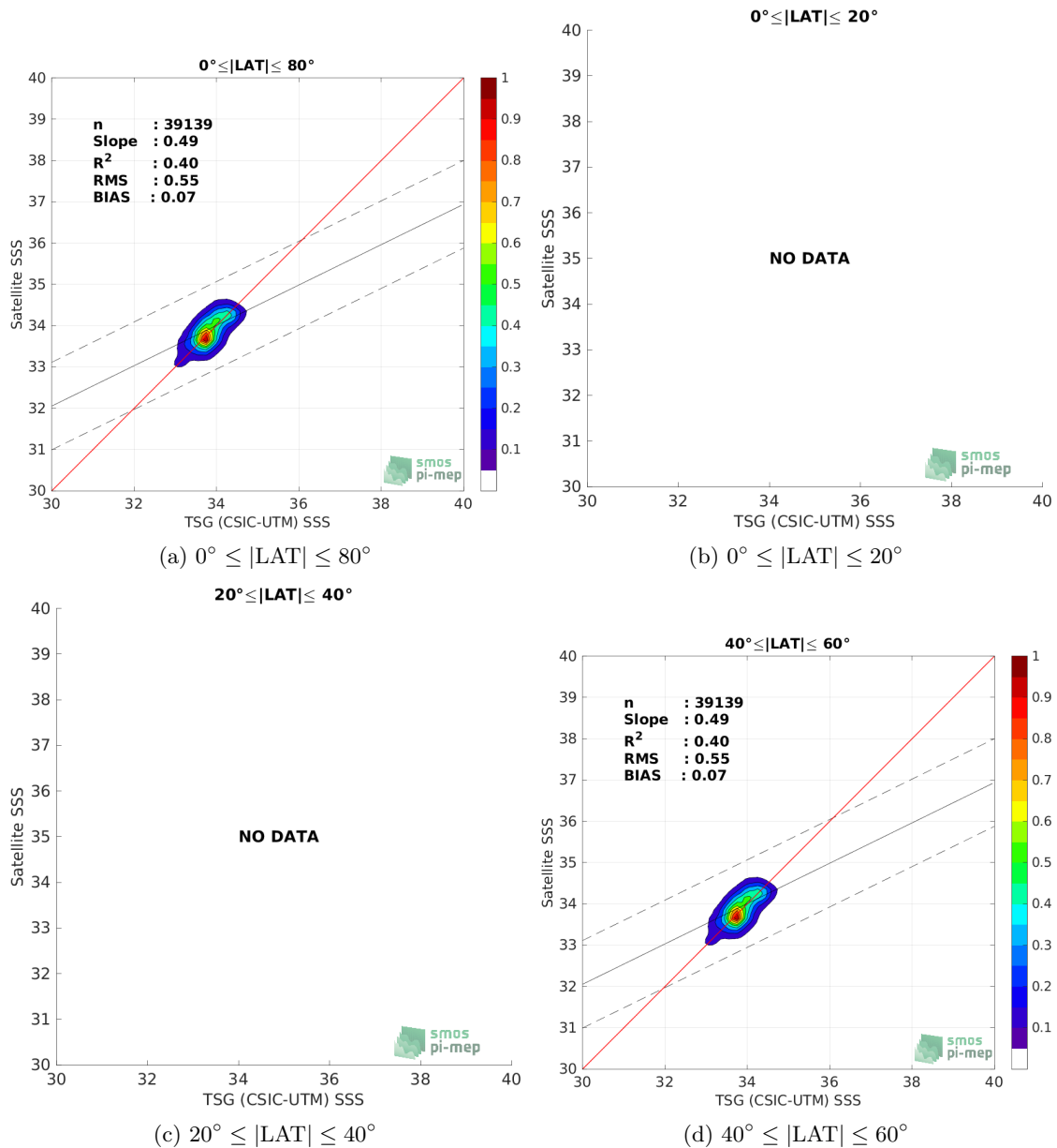
Figure 9: Contour maps of the concentration of Aquarius SSS L3 OR v5 - 7-Day running - Rain mask (NASA-GSFC) SSS (y-axis) versus TSG (CSIC-UTM) SSS (x-axis) at match-up pairs for different latitude bands. For each plot, the red line shows x=y . The black thin and dashed lines indicate a linear fit through the data cloud and the \pm 95\% confidence levels, respectively. The number match-up pairs n , the slope and R^2 coefficient of the linear fit, the root mean square (RMS) and the mean bias between satellite and in situ data are indicated for each latitude band in each plots.
