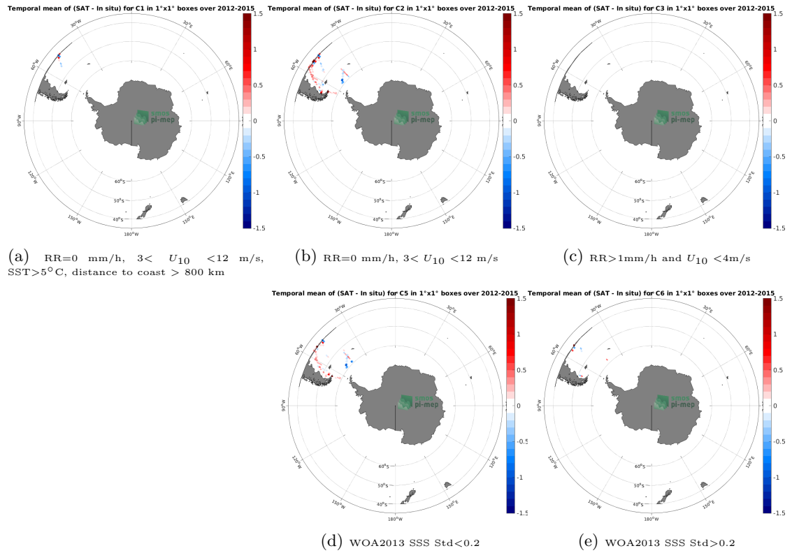
Figure 12: Temporal mean gridded over spatial boxes of size 1^{\circ}\times 1^{\circ} of \Delta\text{SSS} (Aquarius SSS L3 OR v5 - 7-Day running - Rain mask (NASA-GSFC) - TSG (CSIC-UTM)) for 5 different subdatasets corresponding to:RR=0 mm/h, 3 < U_{10} < 12 m/s, SST >5^{\circ}\text{C} , distance to coast > 800 km (a), RR=0 mm/h, 3 < U_{10} < 12 m/s (b), RR >1 mm/h and U_{10} < 4 m/s (c), WOA2013 SSS Std <0.2 (d), WOA2013 SSS Std >0.2 (e).
