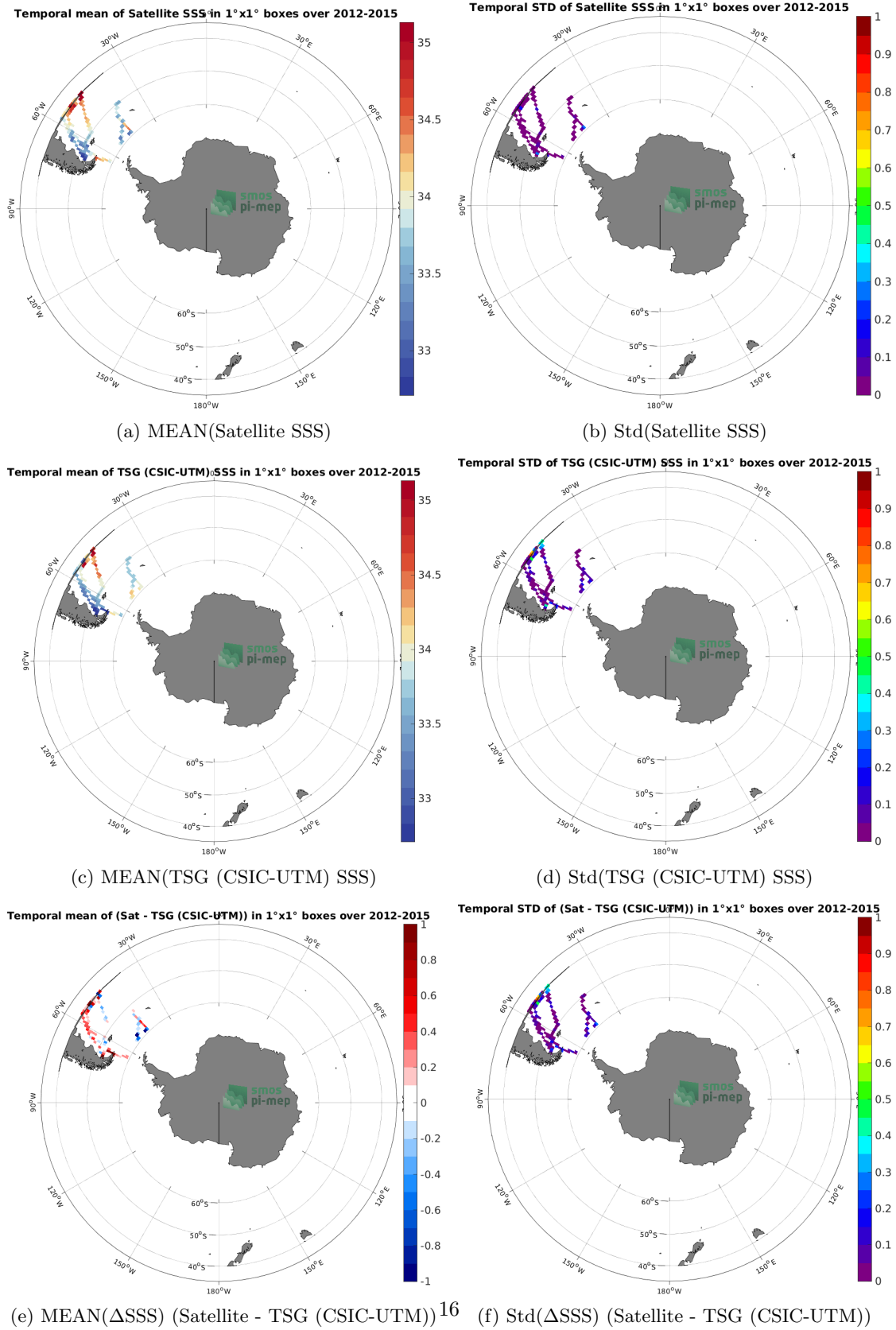
Figure 6: Temporal mean (left) and Std (right) of SSS from Aquarius SSS L3 OR v5 - 7-Day running - Rain mask (NASA-GSFC) (top), TSG (CSIC-UTM) (middle), and of \Delta SSS (Satellite - TSG (CSIC-UTM)). Only match-up pairs are used to generate these maps.
