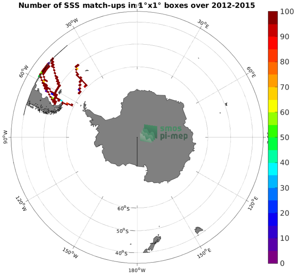
Figure 4: Number of SSS match-ups between TSG (CSIC-UTM) SSS and the Aquarius SSS L3 OR v5 - 7-Day running - Rain mask (NASA-GSFC) SSS product for the Roaring Forties and Furious Fifties Pi-MEP region over 1^\circ \times 1^\circ boxes and for the full satellite product period.
