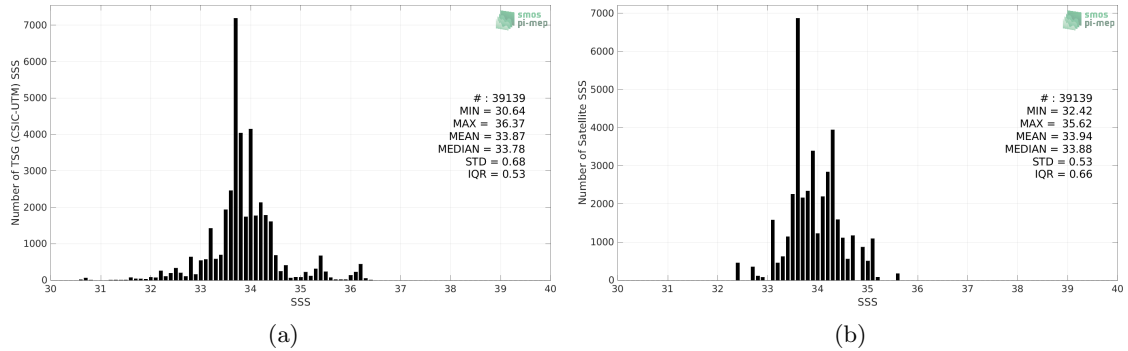
Figure 2: Histograms of SSS from TSG (CSIC-UTM) (a) and Aquarius SSS L3 OR v5 - 7-Day running - Rain mask (NASA-GSFC) (b) considering all match-up pairs per bins of 0.1 over the Roaring Forties and Furious Fifties Pi-MEP region and for the full satellite product period.
