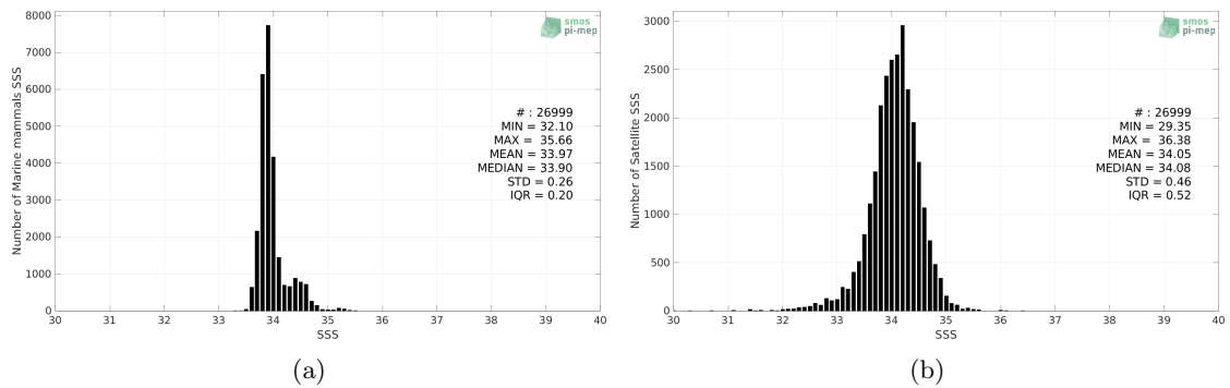
Figure 2: Histograms of SSS from Marine mammals (a) and Aquarius SSS L3 OR v5 - 7-Day running - Rain mask (NASA-GSFC) (b) considering all match-up pairs per bins of 0.1 over the Roaring Forties and Furious Fifties Pi-MEP region and for the full satellite product period.
