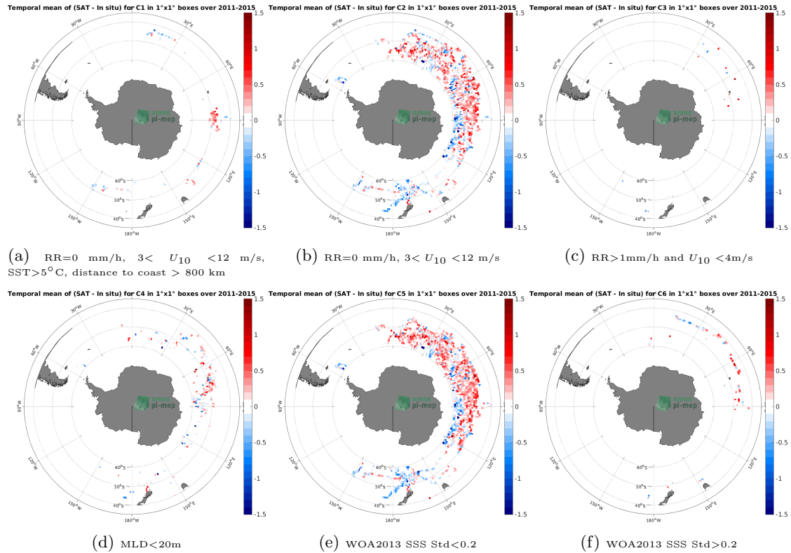
Figure 12: Temporal mean gridded over spatial boxes of size 1^{\circ} \times 1^{\circ} of \Delta\text{SSS} (Aquarius SSS L3 OR v5 - 7-Day running - Rain mask (NASA-GSFC) - Marine mammals) for 6 different subdatasets corresponding to:RR=0 mm/h, 3 < U_{10} < 12 m/s, SST >5^{\circ}\text{C} , distance to coast > 800 km (a), RR=0 mm/h, 3 < U_{10} < 12 m/s (b), RR >1\text{mm/h} and U_{10} < 4\text{m/s} (c),MLD <20\text{m} (d),WOA2013 SSS Std <0.2 (e),WOA2013 SSS Std >0.2 (f).
