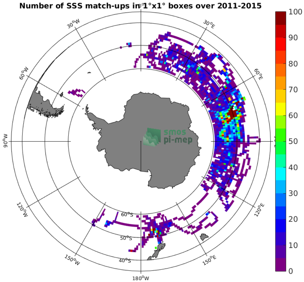
Figure 4: Number of SSS match-ups between Sea mammals SSS and the Aquarius-L3-OR-V5-7DAY-RUNNING-RAIN-MASK-1DEG SSS product for the Roaring Forties and Furious Fifties Pi-MEP region over 1°x1° boxes and for the full satellite product period.
