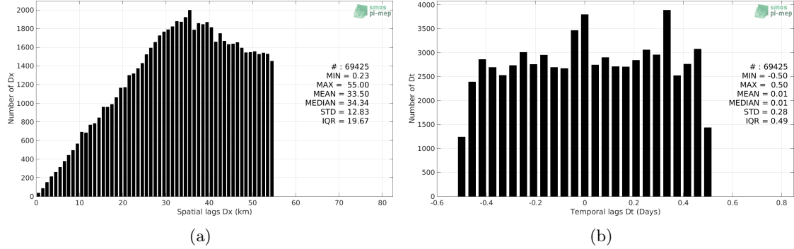
Figure 5: Histograms of the spatial (a) and temporal (b) lags between the time of the Argo measurements and the date of the corresponding Aquarius SSS L3 OR v5 - 7-Day running - Rain mask (NASA-GSFC) SSS product.
