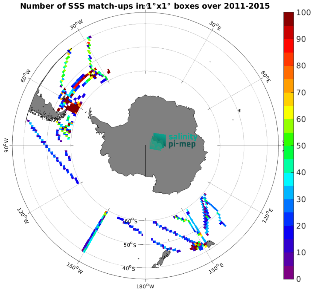
Figure 5: Number of SSS match-ups between TSG (SAMOS) SSS and the Aquarius SSS L3 OR v5 - Monthly (NASA-GSFC) SSS product for the Roaring Forties and Furious Fifties Pi-MEP region over 1^\circ \times 1^\circ boxes and for the full satellite product period.
