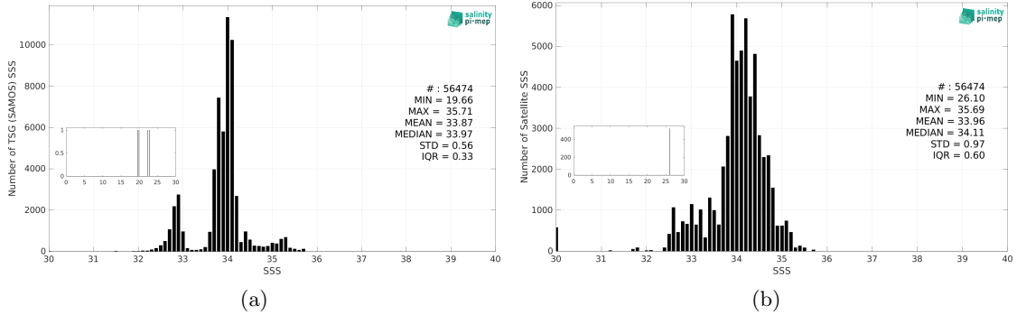
Figure 3: Histograms of SSS from TSG (SAMOS) (a) and Aquarius SSS L3 OR v5 - Monthly (NASA-GSFC) (b) considering all match-up pairs per bins of 0.1 over the Roaring Forties and Furious Fifties Pi-MEP region and for the full satellite product period.
