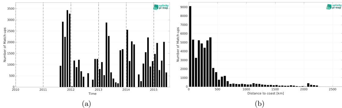
Figure 2: Number of match-ups between TSG (SAMOS) and Aquarius SSS L3 OR v5 - Monthly (NASA-GSFC) SSS as a function of time (a) and as function of the distance to coast (b) over the Roaring Forties and Furious Fifties Pi-MEP region and for the full satellite product period.
