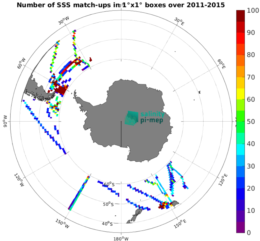
Figure 4: Number of SSS match-ups between TSG (SAMOS) SSS and the Aquarius SSS L3 OR v5 - Monthly (NASA-GSFC) SSS product for the Roaring Forties and Furious Fifties Pi-MEP region over 1^\circ \times 1^\circ boxes and for the full satellite product period.
