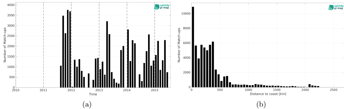
Figure 1: Number of match-ups between TSG (SAMOS) and Aquarius SSS L3 OR v5 - Monthly (NASA-GSFC) SSS as a function of time (a) and as function of the distance to coast (b) over the Roaring Forties and Furious Fifties Pi-MEP region and for the full satellite product period.
