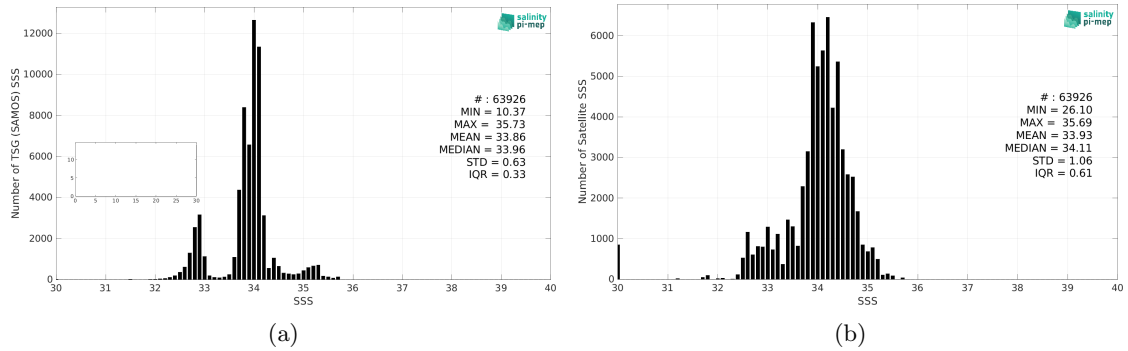
Figure 2: Histograms of SSS from TSG (SAMOS) (a) and Aquarius SSS L3 OR v5 - Monthly (NASA-GSFC) (b) considering all match-up pairs per bins of 0.1 over the Roaring Forties and Furious Fifties Pi-MEP region and for the full satellite product period.
