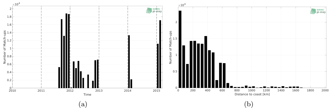
Figure 1: Number of match-ups between TSG (SAMOS) and Aquarius SSS L3 OR v5 - Monthly (NASA-GSFC) SSS as a function of time (a) and as function of the distance to coast (b) over the Roaring Forties and Furious Fifties Pi-MEP region and for the full satellite product period.
