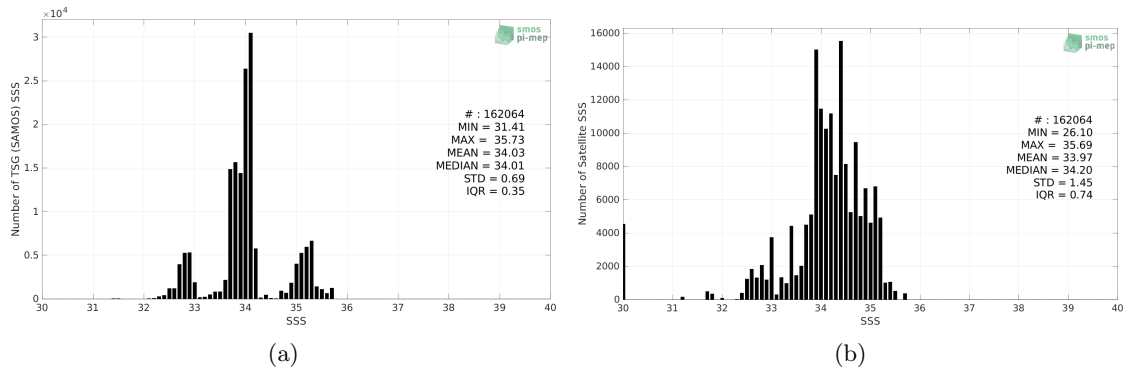
Figure 2: Histograms of SSS from TSG (SAMOS) (a) and Aquarius SSS L3 OR v5 - Monthly (NASA-GSFC) (b) considering all match-up pairs per bins of 0.1 over the Roaring Forties and Furious Fifties Pi-MEP region and for the full satellite product period.
