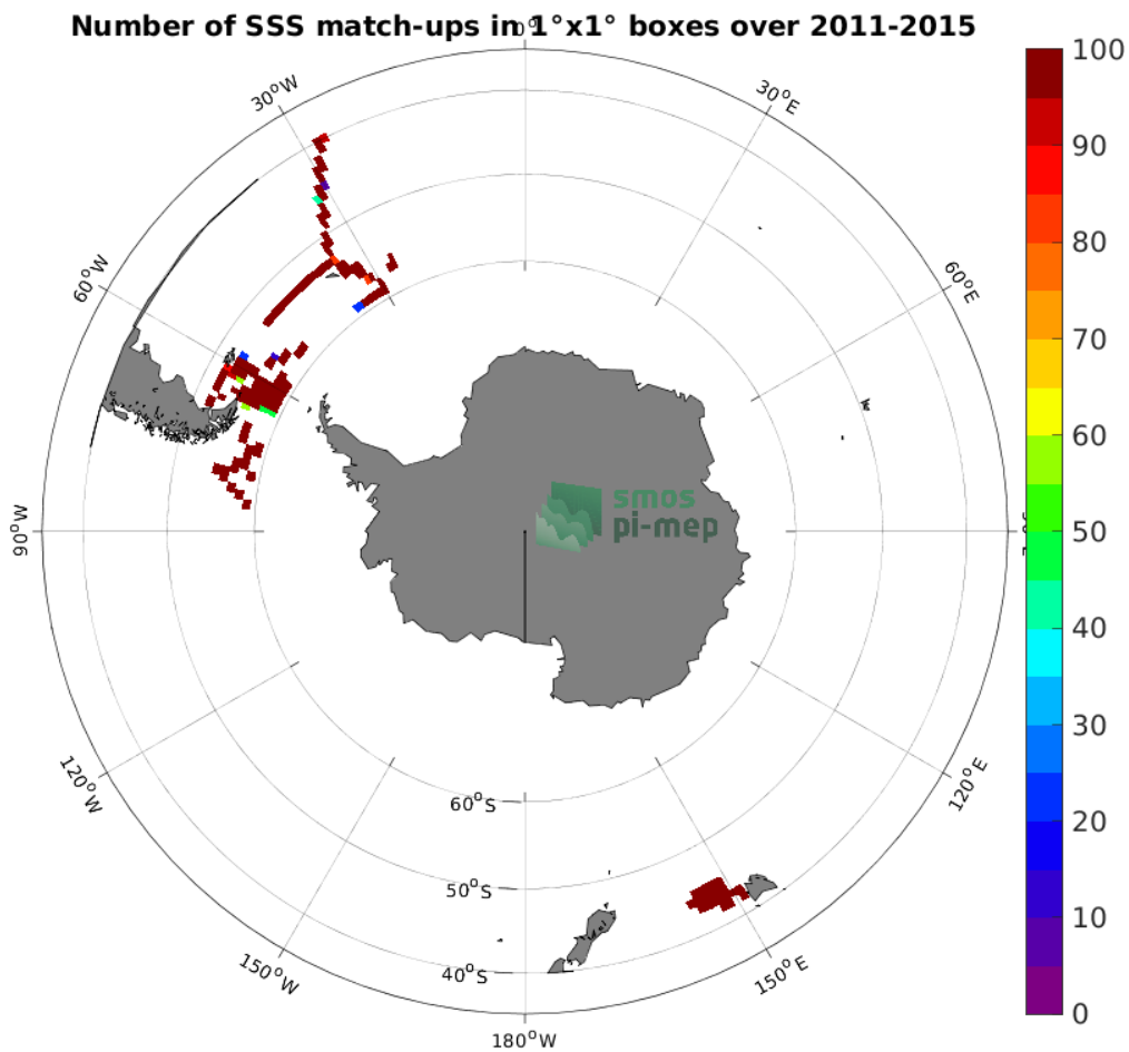
Figure 4: Number of SSS match-ups between TSG (SAMOS) SSS and the Aquarius SSS L3 OR v5 - Monthly (NASA-GSFC) SSS product for the Roaring Forties and Furious Fifties Pi-MEP region over 1^\circ \times 1^\circ boxes and for the full satellite product period.
