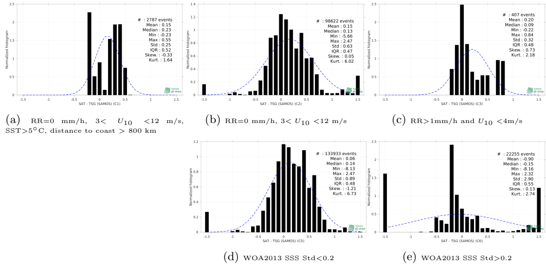
Figure 13: Normalized histogram of \Delta\text{SSS} (Aquarius SSS L3 OR v5 - Monthly (NASA-GSFC) - TSG (SAMOS)) for 5 different subdatasets corresponding to: RR=0 mm/h, 3 < U_{10} < 12 m/s, SST>5°C, distance to coast > 800 km (a), RR=0 mm/h, 3 < U_{10} < 12 m/s (b), RR>1mm/h and U_{10} < 4 m/s (c), WOA2013 SSS Std<0.2 (d), WOA2013 SSS Std>0.2 (e).
