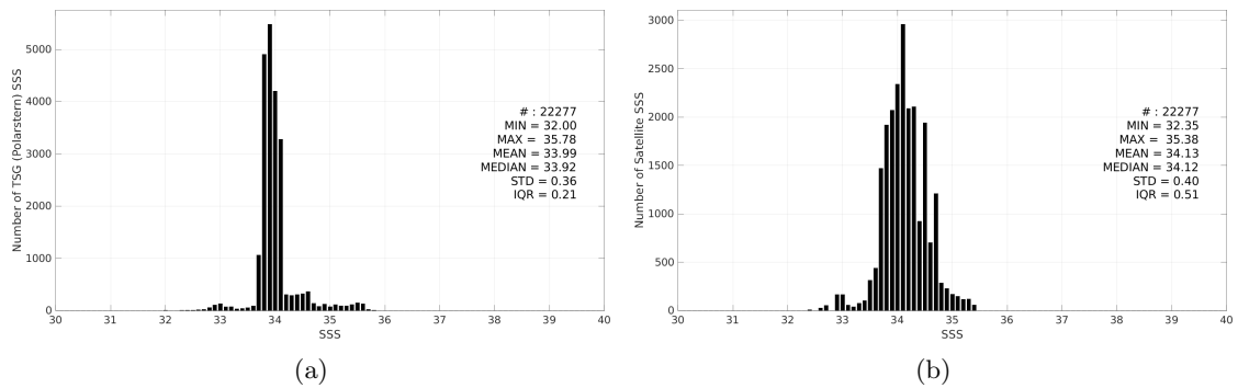
Figure 3: Histograms of SSS from TSG (Polarstern) (a) and Aquarius SSS L3 OR v5 - Monthly (NASA-GSFC) (b) considering all match-up pairs per bins of 0.1 over the Roaring Forties and Furious Fifties Pi-MEP region and for the full satellite product period.
