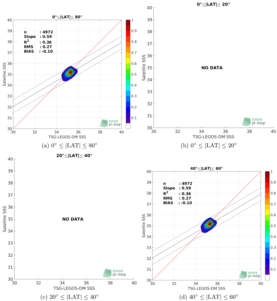
Figure 9: Contour maps of the concentration of Aquarius-L3-OR-V5-MONTHLY SSS (y-axis) versus TSG-LEGOS-DM SSS (x-axis) at match-up pairs for different latitude bands. For each plot, the red line shows x=y . The black thin and dashed lines indicate a linear fit through the data cloud and the \pm 95\% confidence levels, respectively. The number match-up pairs n , the slope and R^2 coefficient of the linear fit, the root mean square (RMS) and the mean bias between satellite and in situ data are indicated for each latitude band in each plots.
