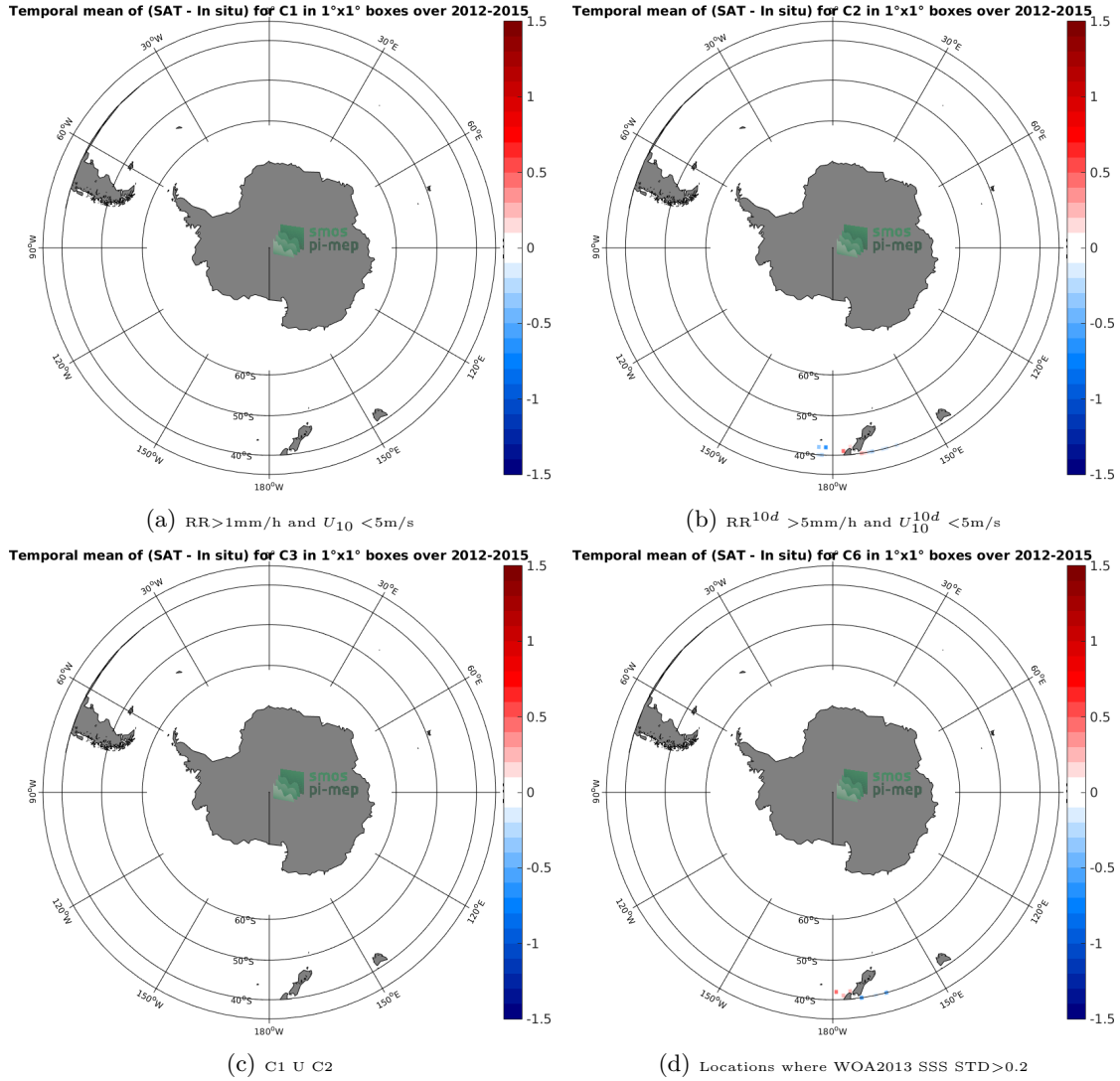
Figure 12: Temporal mean gridded over spatial boxes of size 1^\circ \times 1^\circ of \Delta SSS (Aquarius-L3-OR-V5-MONTHLY - TSG-LEGOS-DM) for 4 different subdatasets corresponding to:RR >1 mm/h and U_{10} < 5 m/s (a), RR 10d > 5 mm/h and U_{10}^{10d} < 5 m/s (b), C1 U C2 (c),Locations where WOA2013 SSS STD > 0.2 (d).
