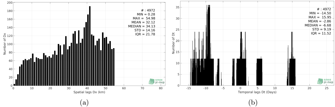
Figure 5: Histograms of the spatial (a) and temporal (b) lags between the time of the TSG-LEGOS-DM measurements and the date of the corresponding Aquarius-L3-OR-V5-MONTHLY SSS product.
