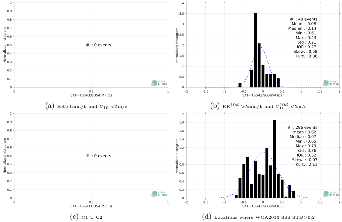
Figure 13: Normalized histogram of \Delta\text{SSS} (Aquarius-L3-OR-V5-MONTHLY - TSG-LEGOS-DM) for 6 different subdatasets corresponding to: RR > 1\text{mm/h} and U_{10} < 5\text{m/s} (a), RR^{10d} > 5\text{mm/h} and U_{10}^{10d} < 5\text{m/s} (b), C1 \cup C2 (c), Locations where WOA2013 SSS STD > 0.2 (d).
