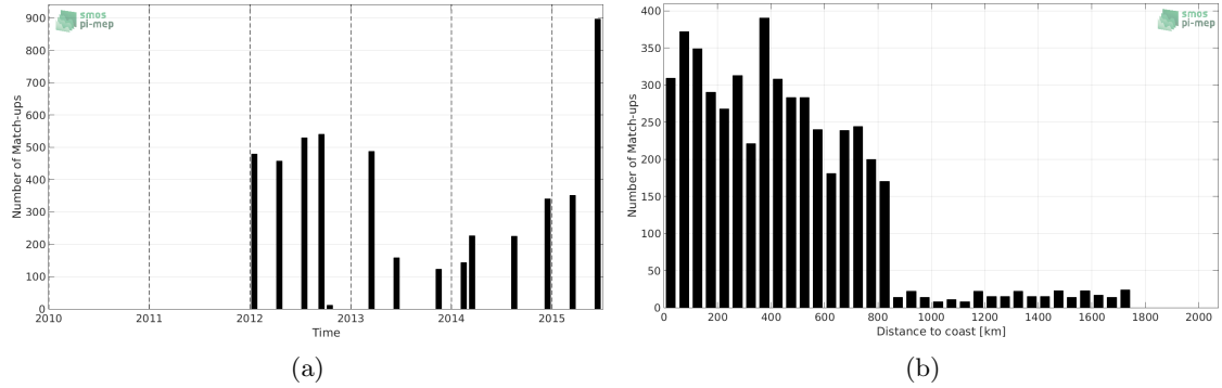
Figure 1: Number of match-ups between TSG-LEGOS-DM and Aquarius-L3-OR-V5-MONTHLY SSS as a function of time (a) and as function of the distance to coast (b) over the Roaring Forties and Furious Fifties Pi-MEP region and for the full satellite product period.
