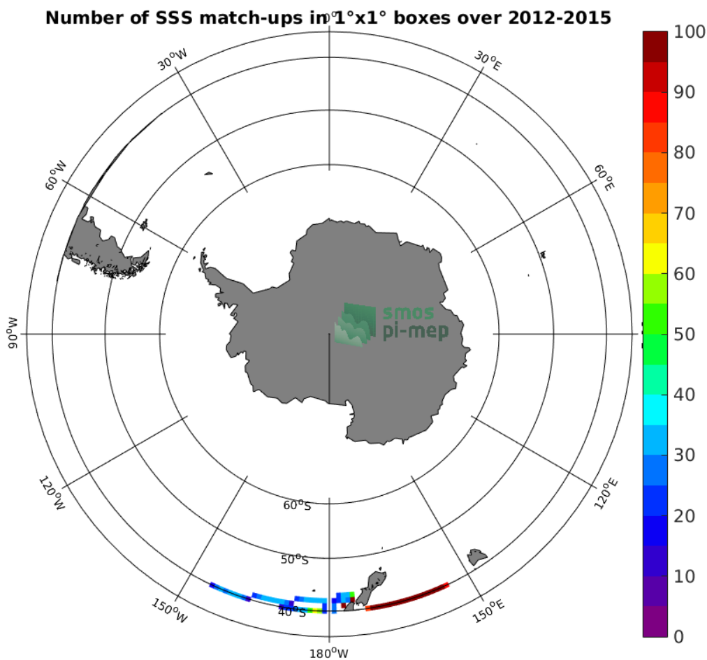
Figure 4: Number of SSS match-ups between TSG-LEGOS-DM SSS and the Aquarius-L3-OR-V5-MONTHLY SSS product for the Roaring Forties and Furious Fifties Pi-MEP region over 1°x1° boxes and for the full satellite product period.
