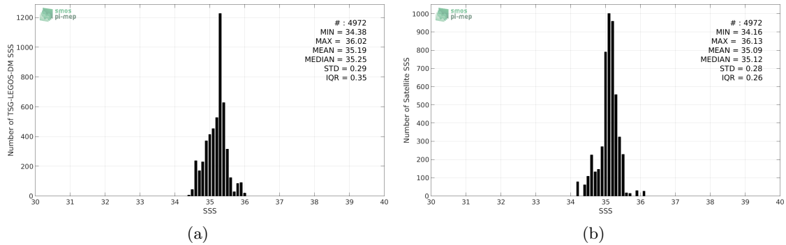
Figure 2: Histograms of SSS from TSG-LEGOS-DM (a) and Aquarius-L3-OR-V5-MONTHLY (b) considering all match-up pairs per bins of 0.1 over the Roaring Forties and Furious Fifties Pi-MEP region and for the full satellite product period.
