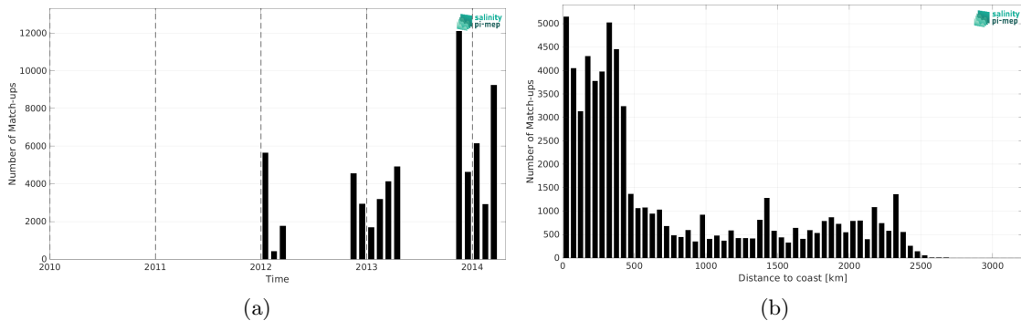
Figure 2: Number of match-ups between TSG (GOSUD-Sailing-ship) and Aquarius SSS L3 OR v5 - Monthly (NASA-GSFC) SSS as a function of time (a) and as function of the distance to coast (b) over the Roaring Forties and Furious Fifties Pi-MEP region and for the full satellite product period.
