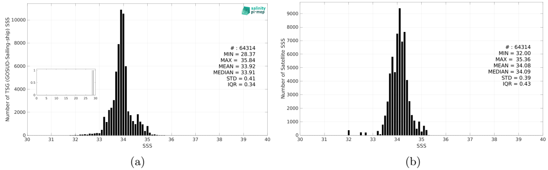
Figure 3: Histograms of SSS from TSG (GOSUD-Sailing-ship) (a) and Aquarius SSS L3 OR v5 - Monthly (NASA-GSFC) (b) considering all match-up pairs per bins of 0.1 over the Roaring Forties and Furious Fifties Pi-MEP region and for the full satellite product period.
