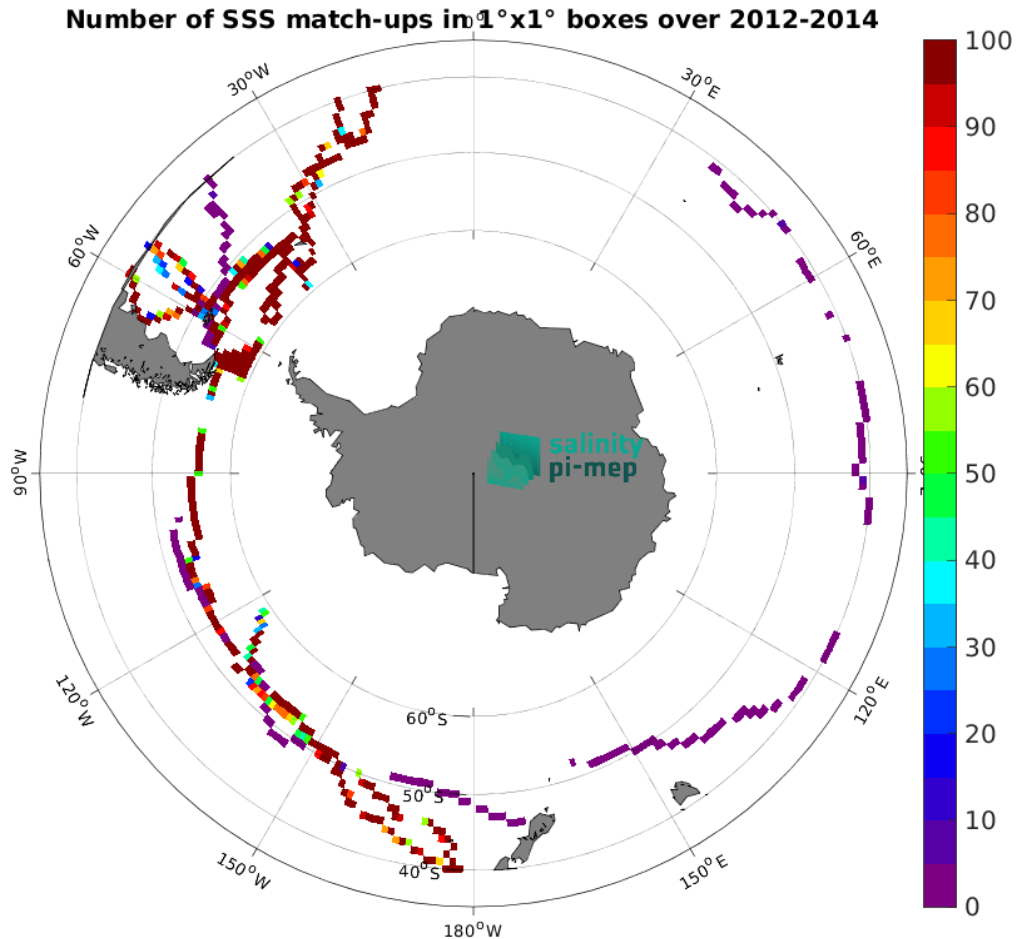
Figure 5: Number of SSS match-ups between TSG (GOSUD-Sailing-ship) SSS and the Aquarius SSS L3 OR v5 - Monthly (NASA-GSFC) SSS product for the Roaring Forties and Furious Fifties Pi-MEP region over 1^\circ \times 1^\circ boxes and for the full satellite product period.
