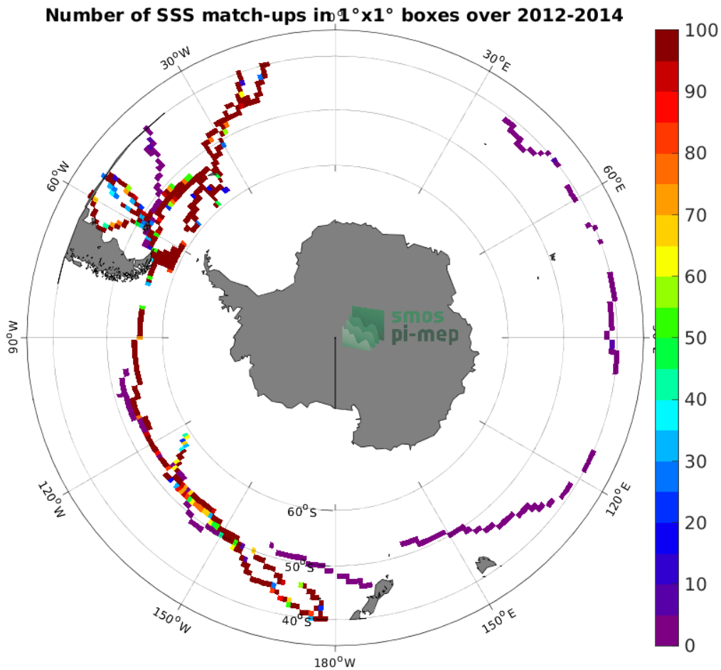
Figure 4: Number of SSS match-ups between TSG (GOSUD-Sailing-ship) SSS and the Aquarius SSS L3 OR v5 - Monthly (NASA-GSFC) SSS product for the Roaring Forties and Furious Fifties Pi-MEP region over 1^\circ \times 1^\circ boxes and for the full satellite product period.
