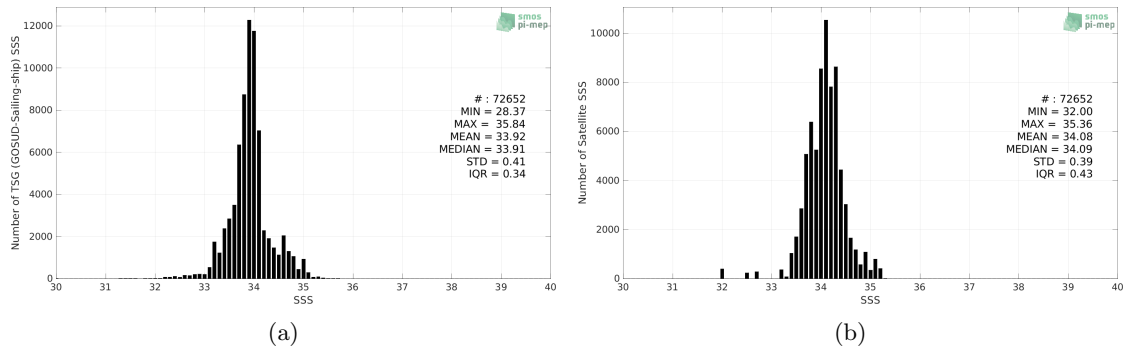
Figure 2: Histograms of SSS from TSG (GOSUD-Sailing-ship) (a) and Aquarius SSS L3 OR v5 - Monthly (NASA-GSFC) (b) considering all match-up pairs per bins of 0.1 over the Roaring Forties and Furious Fifties Pi-MEP region and for the full satellite product period.
