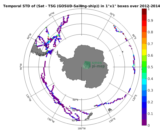
(f) Std( \Delta SSS) (Satellite - TSG (GOSUD-Sailing-ship))
