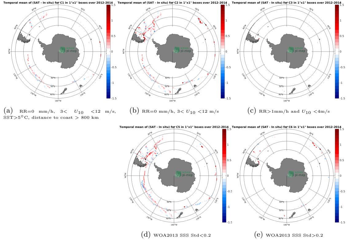
Figure 12: Temporal mean gridded over spatial boxes of size 1^\circ \times 1^\circ of \Delta\text{SSS} (Aquarius SSS L3 OR v5 - Monthly (NASA-GSFC) - TSG (GOSUD-Sailing-ship)) for 5 different subdatasets corresponding to: RR=0 mm/h, 3 < U_{10} < 12 m/s, SST > 5^\circ\text{C} , distance to coast > 800 km (a), RR=0 mm/h, 3 < U_{10} < 12 m/s (b), RR > 1 mm/h and U_{10} < 4 m/s (c), WOA2013 SSS Std < 0.2 (d), WOA2013 SSS Std > 0.2 (e).
