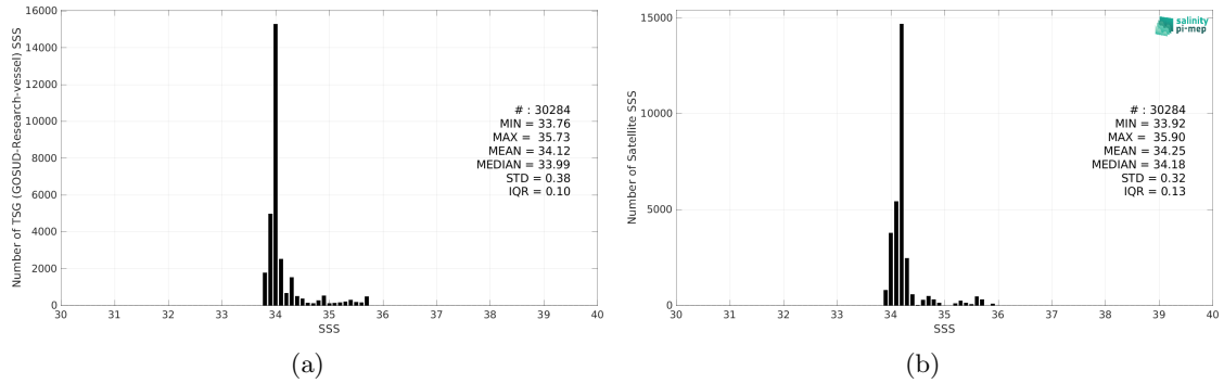
Figure 2: Histograms of SSS from TSG (GOSUD-Research-vessel) (a) and Aquarius SSS L3 OR v5 - Monthly (NASA-GSFC) (b) considering all match-up pairs per bins of 0.1 over the Roaring Forties and Furious Fifties Pi-MEP region and for the full satellite product period.
