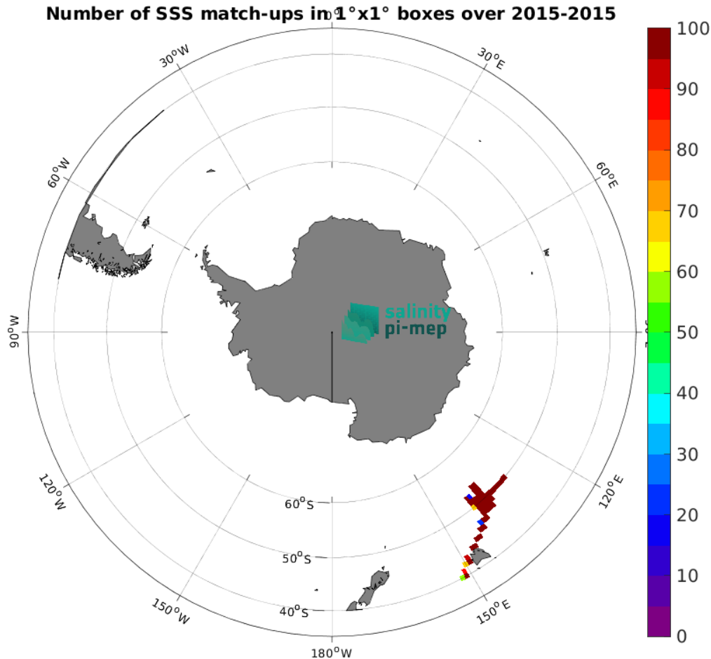
Figure 4: Number of SSS match-ups between TSG (GOSUD-Research-vessel) SSS and the Aquarius SSS L3 OR v5 - Monthly (NASA-GSFC) SSS product for the Roaring Forties and Furious Fifties Pi-MEP region over 1^\circ \times 1^\circ boxes and for the full satellite product period.
