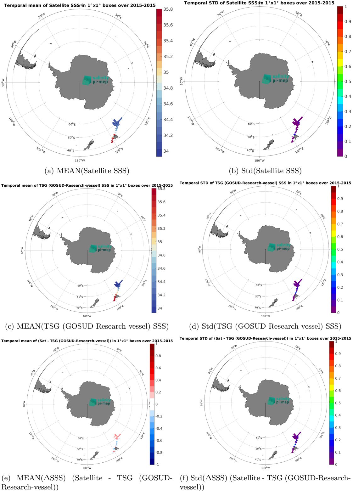
Figure 6: Temporal mean (left) and Std (right) of SSS from Aquarius SSS L3 OR v5 - Monthly (NASA-GSFC) (top), TSG (GOSUD-Research-vessel) (middle), and of \Delta SSS (Satellite - TSG (GOSUD-Research-vessel)). Only match-up pairs are used to generate these maps.
