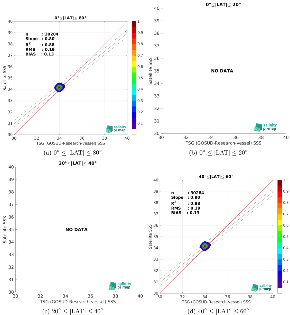
Figure 9: Contour maps of the concentration of Aquarius SSS L3 OR v5 - Monthly (NASA-GSFC) SSS (y-axis) versus TSG (GOSUD-Research-vessel) SSS (x-axis) at match-up pairs for different latitude bands. For each plot, the red line shows x=y . The black thin and dashed lines indicate a linear fit through the data cloud and the \pm 95\% confidence levels, respectively. The number match-up pairs n , the slope and R^2 coefficient of the linear fit, the root mean square (RMS) and the mean bias between satellite and in situ data are indicated for each latitude band in each plots.
