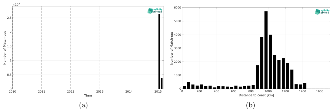
Figure 1: Number of match-ups between TSG (GOSUD-Research-vessel) and Aquarius SSS L3 OR v5 - Monthly (NASA-GSFC) SSS as a function of time (a) and as function of the distance to coast (b) over the Roaring Forties and Furious Fifties Pi-MEP region and for the full satellite product period.
