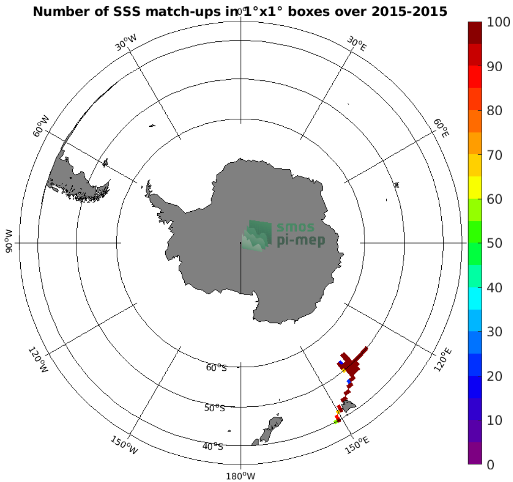
Figure 4: Number of SSS match-ups between TSG (GOSUD-Research-vessel) SSS and the Aquarius SSS L3 OR v5 - Monthly (NASA-GSFC) SSS product for the Roaring Forties and Furious Fifties Pi-MEP region over 1^\circ \times 1^\circ boxes and for the full satellite product period.
