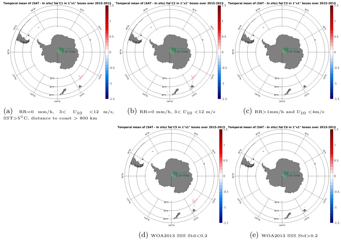
Figure 12: Temporal mean gridded over spatial boxes of size 1°x1° of \Delta SSS (Aquarius SSS L3 OR v5 - Monthly (NASA-GSFC) - TSG (GOSUD-Research-vessel)) for 5 different subdatasets corresponding to:RR=0 mm/h, 3 < U_{10} < 12 m/s, SST>5°C, distance to coast > 800 km (a), RR=0 mm/h, 3 < U_{10} < 12 m/s (b), RR>1mm/h and U_{10} < 4 m/s (c), WOA2013 SSS Std<0.2 (d), WOA2013 SSS Std>0.2 (e).
