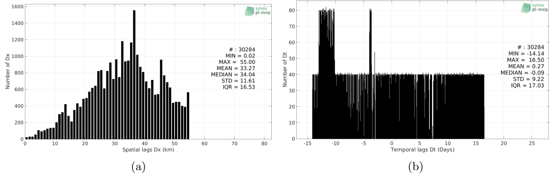
Figure 5: Histograms of the spatial (a) and temporal (b) lags between the time of the TSG (GOSUD-Research-vessel) measurements and the date of the corresponding Aquarius SSS L3 OR v5 - Monthly (NASA-GSFC) SSS product.
