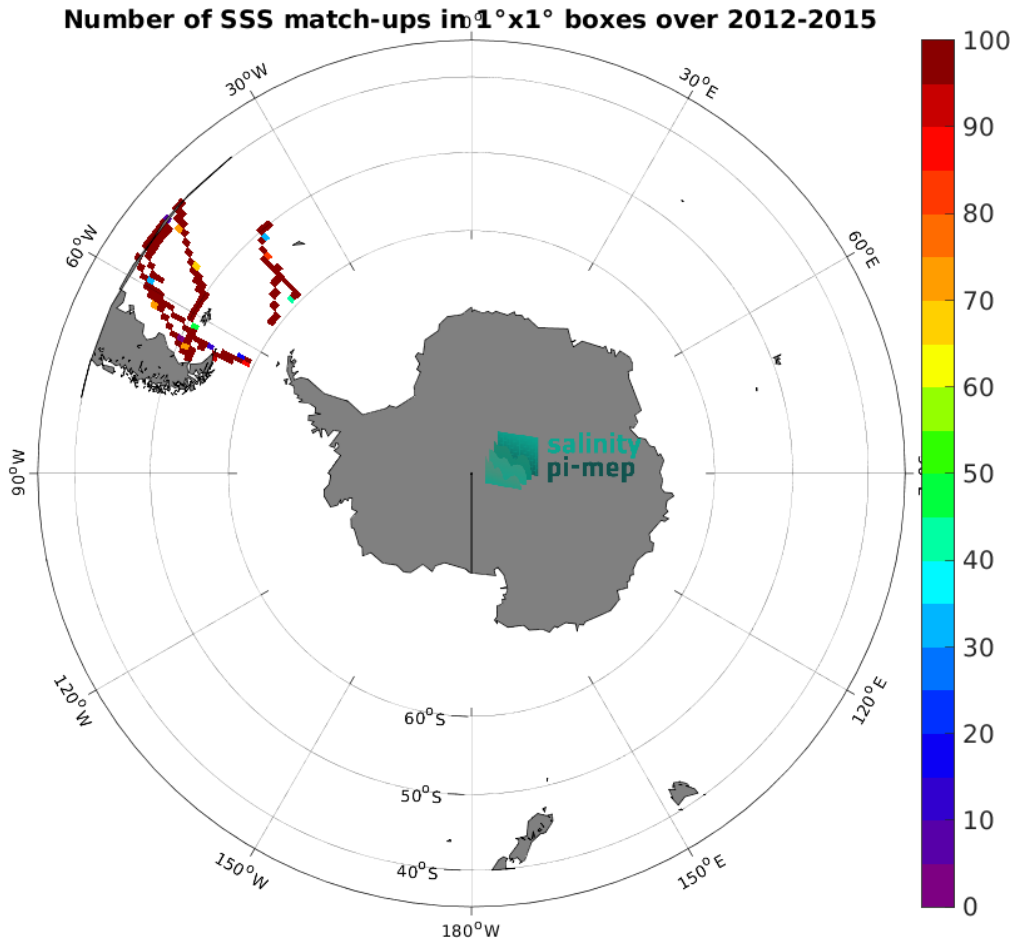
Figure 5: Number of SSS match-ups between TSG (CSIC-UTM) SSS and the Aquarius SSS L3 OR v5 - Monthly (NASA-GSFC) SSS product for the Roaring Forties and Furious Fifties Pi-MEP region over 1^\circ \times 1^\circ boxes and for the full satellite product period.
