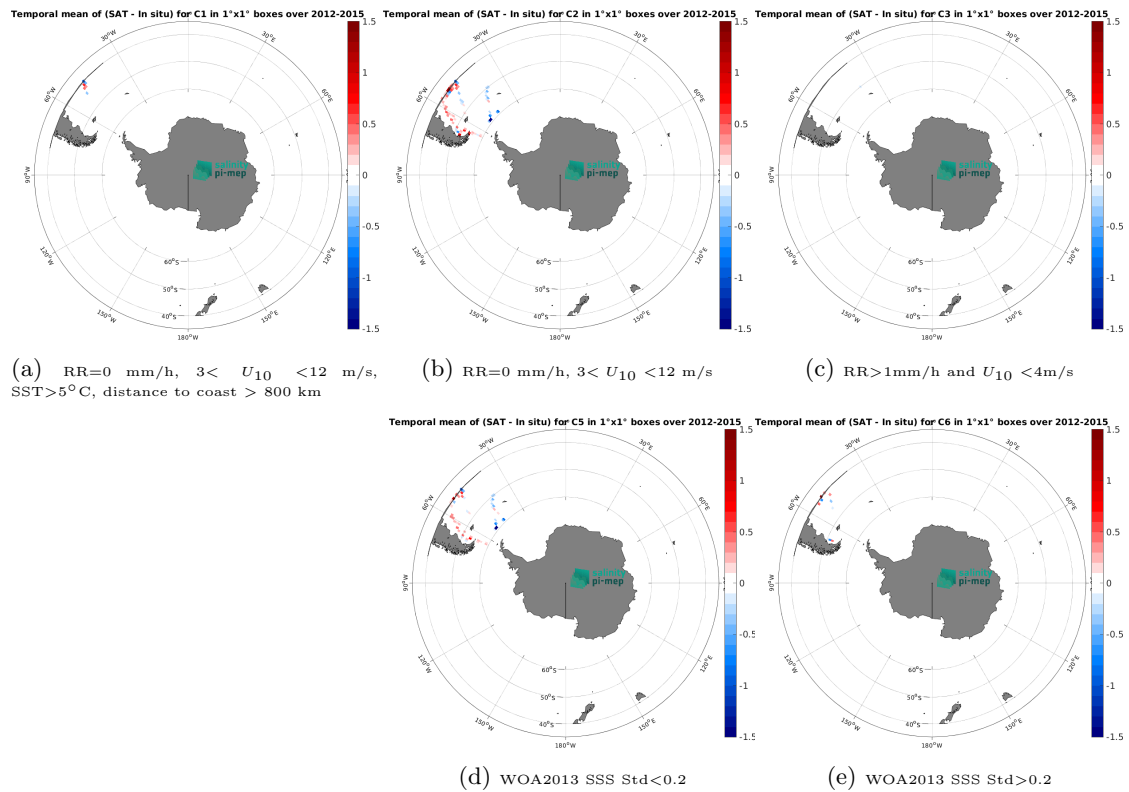
Figure 14: Temporal mean gridded over spatial boxes of size 1^\circ \times 1^\circ of \Delta SSS (Aquarius SSS L3 OR v5 - Monthly (NASA-GSFC) - TSG (CSIC-UTM)) for 5 different subdatasets corresponding to:RR=0 mm/h, 3 < U_{10} < 12 m/s, SST>5°C, distance to coast > 800 km (a), RR=0 mm/h, 3 < U_{10} < 12 m/s (b), RR>1mm/h and U_{10} < 4 m/s (c), WOA2013 SSS Std<0.2 (d), WOA2013 SSS Std>0.2 (e).
