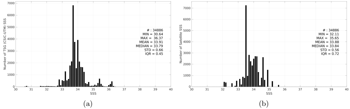
Figure 3: Histograms of SSS from TSG (CSIC-UTM) (a) and Aquarius SSS L3 OR v5 - Monthly (NASA-GSFC) (b) considering all match-up pairs per bins of 0.1 over the Roaring Forties and Furious Fifties Pi-MEP region and for the full satellite product period.
