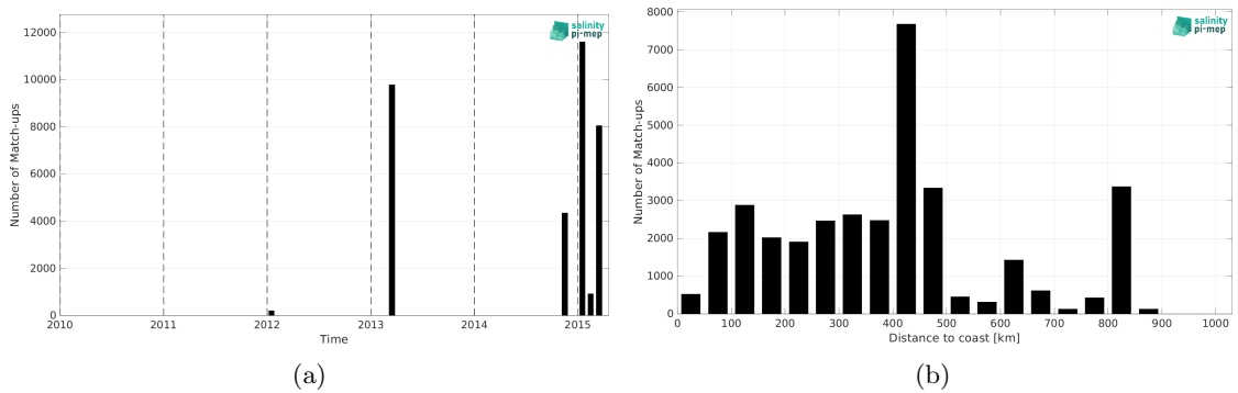
Figure 2: Number of match-ups between TSG (CSIC-UTM) and Aquarius SSS L3 OR v5 - Monthly (NASA-GSFC) SSS as a function of time (a) and as function of the distance to coast (b) over the Roaring Forties and Furious Fifties Pi-MEP region and for the full satellite product period.
