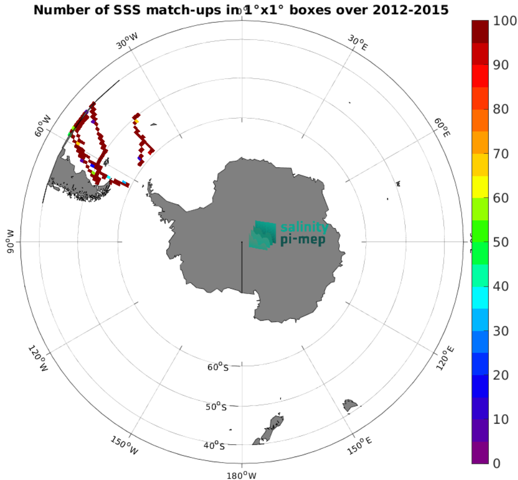
Figure 4: Number of SSS match-ups between TSG (CSIC-UTM) SSS and the Aquarius SSS L3 OR v5 - Monthly (NASA-GSFC) SSS product for the Roaring Forties and Furious Fifties Pi-MEP region over 1^\circ \times 1^\circ boxes and for the full satellite product period.
