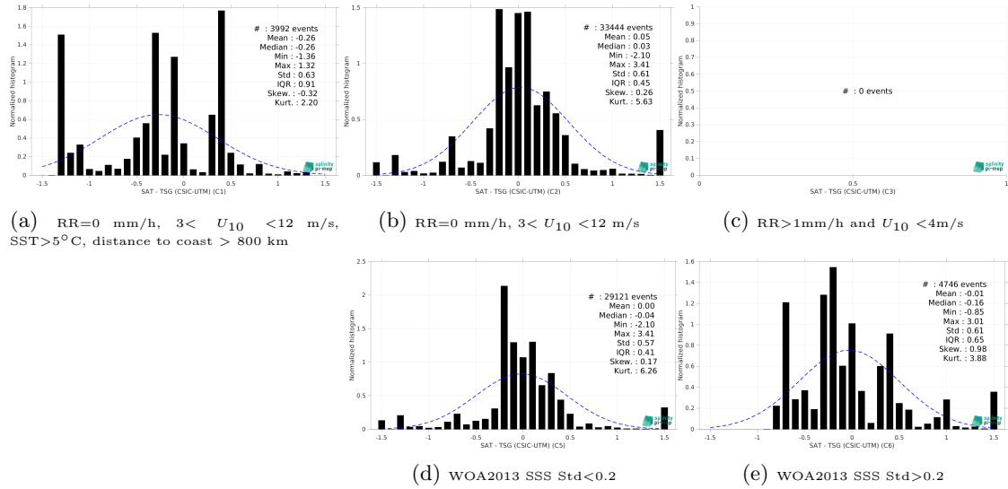
Figure 13: Normalized histogram of \Delta SSS (Aquarius SSS L3 OR v5 - Monthly (NASA-GSFC) - TSG (CSIC-UTM)) for 5 different subdatasets corresponding to: RR=0 mm/h, 3 < U_{10} < 12 m/s, SST > 5°C, distance to coast > 800 km (a), RR=0 mm/h, 3 < U_{10} < 12 m/s (b), RR > 1mm/h and U_{10} < 4 m/s (c), WOA2013 SSS Std < 0.2 (d), WOA2013 SSS Std > 0.2 (e).
