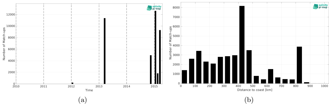
Figure 1: Number of match-ups between TSG (CSIC-UTM) and Aquarius SSS L3 OR v5 - Monthly (NASA-GSFC) SSS as a function of time (a) and as function of the distance to coast (b) over the Roaring Forties and Furious Fifties Pi-MEP region and for the full satellite product period.
