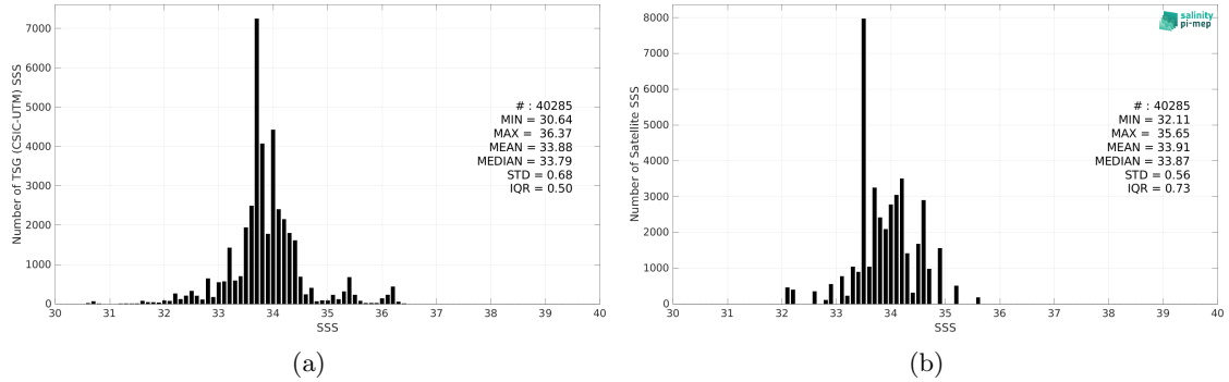
Figure 2: Histograms of SSS from TSG (CSIC-UTM) (a) and Aquarius SSS L3 OR v5 - Monthly (NASA-GSFC) (b) considering all match-up pairs per bins of 0.1 over the Roaring Forties and Furious Fifties Pi-MEP region and for the full satellite product period.
