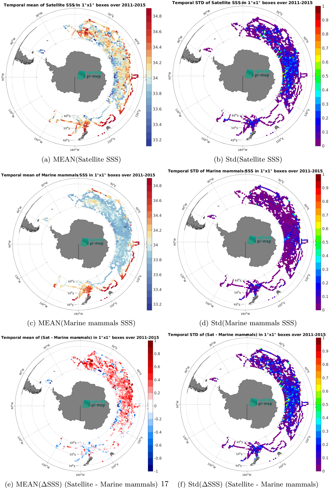
Figure 7: Temporal mean (left) and Std (right) of SSS from Aquarius SSS L3 OR v5 - Monthly (NASA-GSFC) (top), Marine mammals (middle), and of \Delta SSS (Satellite - Marine mammals). Only match-up pairs are used to generate these maps.
