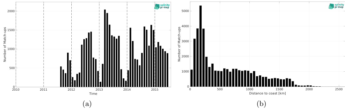
Figure 2: Number of match-ups between Marine mammals and Aquarius SSS L3 OR v5 - Monthly (NASA-GSFC) SSS as a function of time (a) and as function of the distance to coast (b) over the Roaring Forties and Furious Fifties Pi-MEP region and for the full satellite product period.
