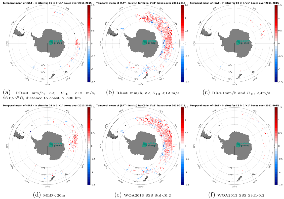
Figure 14: Temporal mean gridded over spatial boxes of size 1^\circ \times 1^\circ of \Delta\text{SSS} (Aquarius SSS L3 OR v5 - Monthly (NASA-GSFC) - Marine mammals) for 6 different subdatasets corresponding to:RR=0 mm/h, 3 < U_{10} < 12 m/s, SST>5°C, distance to coast > 800 km (a), RR=0 mm/h, 3 < U_{10} < 12 m/s (b), RR>1mm/h and U_{10} < 4 m/s (c),MLD<20m (d),WOA2013 SSS Std<0.2 (e),WOA2013 SSS Std>0.2 (f).
