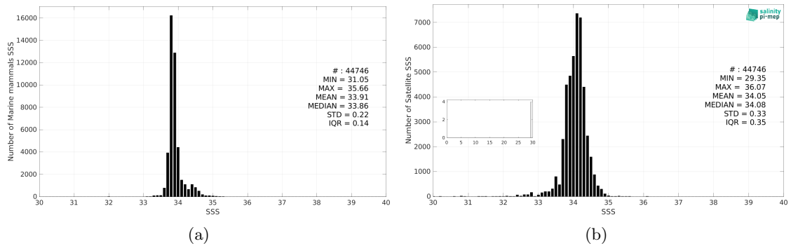
Figure 3: Histograms of SSS from Marine mammals (a) and Aquarius SSS L3 OR v5 - Monthly (NASA-GSFC) (b) considering all match-up pairs per bins of 0.1 over the Roaring Forties and Furious Fifties Pi-MEP region and for the full satellite product period.
