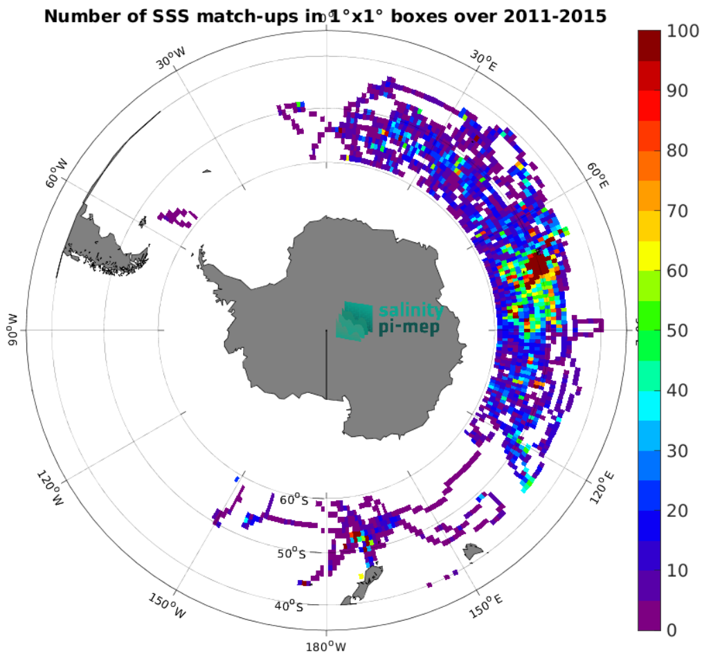
Figure 5: Number of SSS match-ups between Marine mammals SSS and the Aquarius SSS L3 OR v5 - Monthly (NASA-GSFC) SSS product for the Roaring Forties and Furious Fifties Pi-MEP region over 1^\circ \times 1^\circ boxes and for the full satellite product period.
