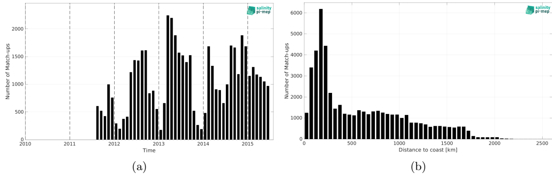
Figure 1: Number of match-ups between Marine mammals and Aquarius SSS L3 OR v5 - Monthly (NASA-GSFC) SSS as a function of time (a) and as function of the distance to coast (b) over the Roaring Forties and Furious Fifties Pi-MEP region and for the full satellite product period.
