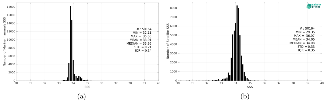
Figure 2: Histograms of SSS from Marine mammals (a) and Aquarius SSS L3 OR v5 - Monthly (NASA-GSFC) (b) considering all match-up pairs per bins of 0.1 over the Roaring Forties and Furious Fifties Pi-MEP region and for the full satellite product period.
