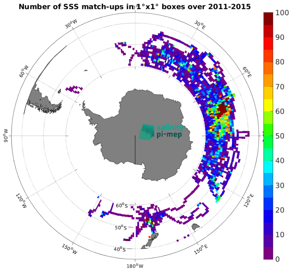
Figure 4: Number of SSS match-ups between Marine mammals SSS and the Aquarius SSS L3 OR v5 - Monthly (NASA-GSFC) SSS product for the Roaring Forties and Furious Fifties Pi-MEP region over 1^\circ \times 1^\circ boxes and for the full satellite product period.
