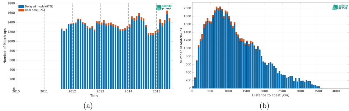
Figure 2: Number of match-ups between Argo and Aquarius SSS L3 OR v5 - Monthly (NASA-GSFC) SSS as a function of time (a) and as function of the distance to coast (b) over the Roaring Forties and Furious Fifties Pi-MEP region and for the full satellite product period.
