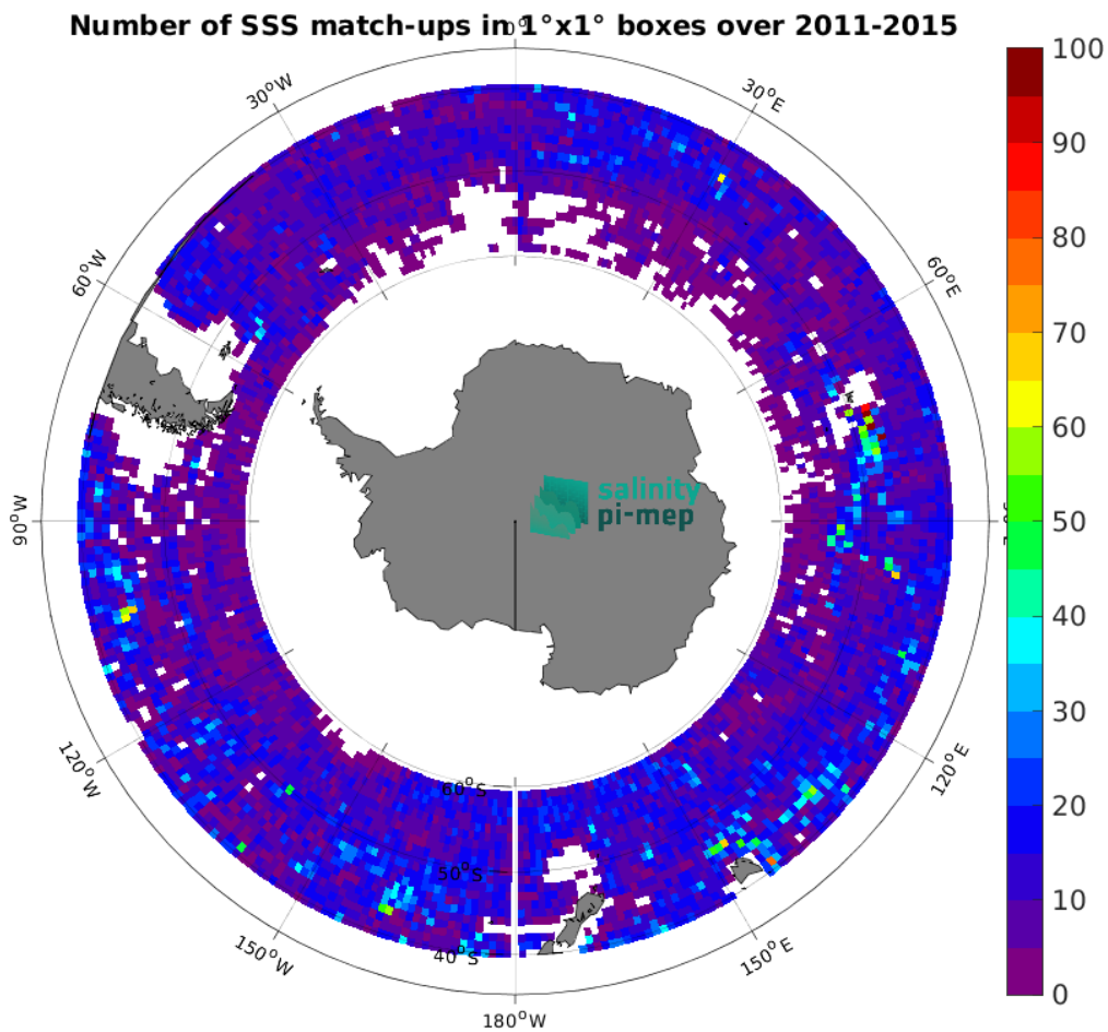
Figure 5: Number of SSS match-ups between Argo SSS and the Aquarius SSS L3 OR v5 - Monthly (NASA-GSFC) SSS product for the Roaring Forties and Furious Fifties Pi-MEP region over 1^\circ \times 1^\circ boxes and for the full satellite product period.
