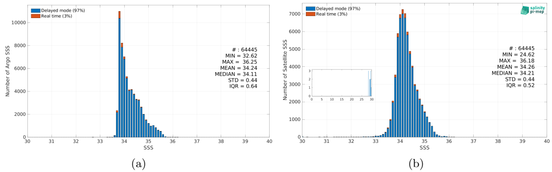
Figure 3: Histograms of SSS from Argo (a) and Aquarius SSS L3 OR v5 - Monthly (NASA-GSFC) (b) considering all match-up pairs per bins of 0.1 over the Roaring Forties and Furious Fifties Pi-MEP region and for the full satellite product period.
