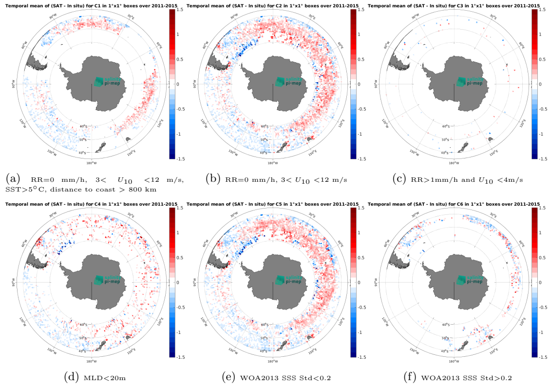
Figure 14: Temporal mean gridded over spatial boxes of size 1^\circ \times 1^\circ of \Delta\text{SSS} (Aquarius SSS L3 OR v5 - Monthly (NASA-GSFC) - Argo) for 6 different subdatasets corresponding to:RR=0 mm/h, 3 < U_{10} < 12 m/s, SST>5°C, distance to coast > 800 km (a), RR=0 mm/h, 3 < U_{10} < 12 m/s (b), RR>1mm/h and U_{10} < 4 m/s (c),MLD<20m (d),WOA2013 SSS Std<0.2 (e),WOA2013 SSS Std>0.2 (f).
