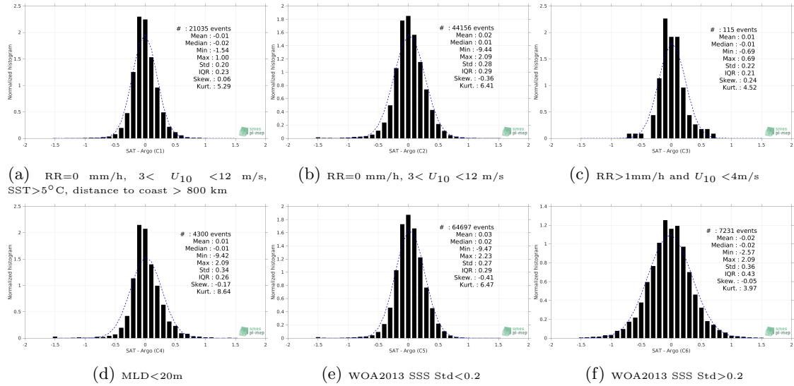
Figure 13: Normalized histogram of \Delta\text{SSS} (Aquarius SSS L3 OR v5 - Monthly (NASA-GSFC) - Argo) for 6 different subdatasets corresponding to: RR=0 mm/h, 3 < U_{10} < 12 m/s, SST>5°C, distance to coast > 800 km (a), RR=0 mm/h, 3 < U_{10} < 12 m/s (b), RR>1mm/h and U_{10} < 4 m/s (c), MLD<20m (d), WOA2013 SSS Std<0.2 (e), WOA2013 SSS Std>0.2 (f).
