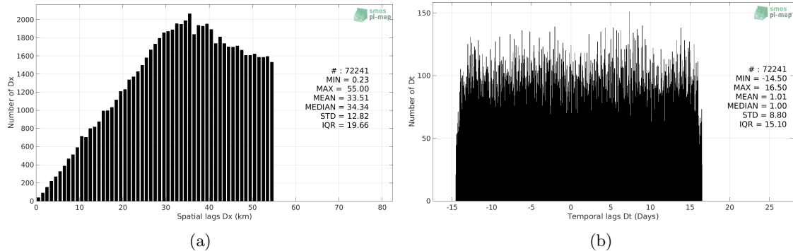
Figure 5: Histograms of the spatial (a) and temporal (b) lags between the time of the Argo measurements and the date of the corresponding Aquarius SSS L3 OR v5 - Monthly (NASA-GSFC) SSS product.
