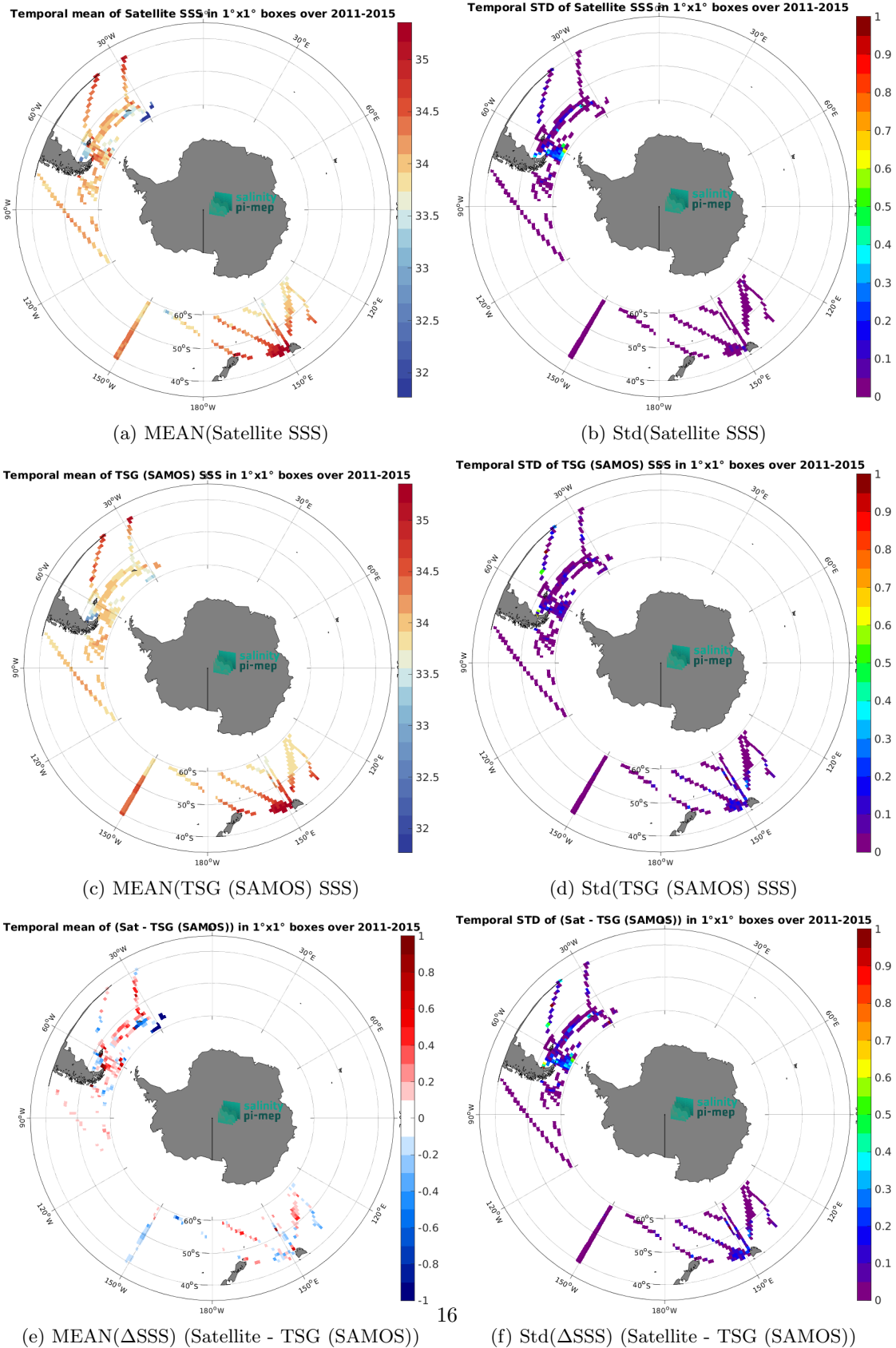
Figure 7: Temporal mean (left) and Std (right) of SSS from Aquarius SSS L3 OR v5 - Monthly - Rain mask (NASA-GSFC) (top), TSG (SAMOS) (middle), and of \Delta SSS (Satellite - TSG (SAMOS)). Only match-up pairs are used to generate these maps.
