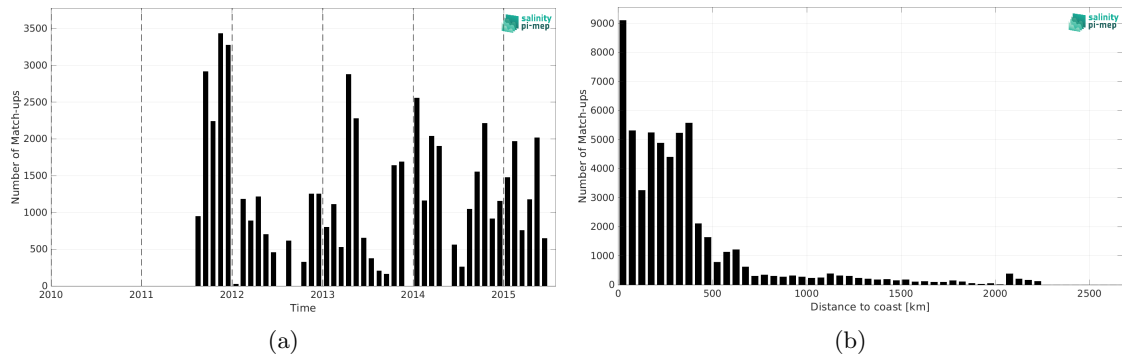
Figure 2: Number of match-ups between TSG (SAMOS) and Aquarius SSS L3 OR v5 - Monthly - Rain mask (NASA-GSFC) SSS as a function of time (a) and as function of the distance to coast (b) over the Roaring Forties and Furious Fifties Pi-MEP region and for the full satellite product period.
