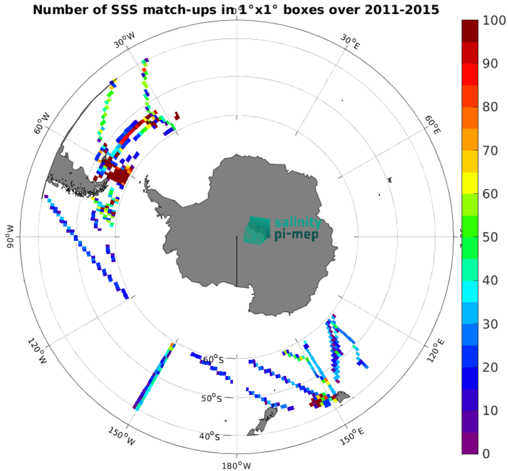
Figure 5: Number of SSS match-ups between TSG (SAMOS) SSS and the Aquarius SSS L3 OR v5 - Monthly - Rain mask (NASA-GSFC) SSS product for the Roaring Forties and Furious Fifties Pi-MEP region over 1^\circ \times 1^\circ boxes and for the full satellite product period.
