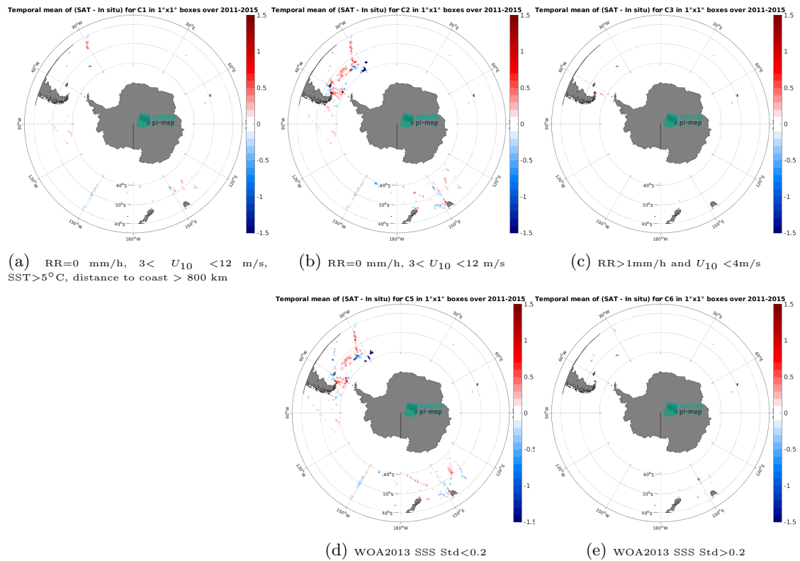
Figure 14: Temporal mean gridded over spatial boxes of size 1^\circ \times 1^\circ of \Delta SSS (Aquarius SSS L3 OR v5 - Monthly - Rain mask (NASA-GSFC) - TSG (SAMOS)) for 5 different subdatasets corresponding to:RR=0 mm/h, 3 < U_{10} < 12 m/s, SST >5^\circ\text{C} , distance to coast > 800 km (a), RR=0 mm/h, 3 < U_{10} < 12 m/s (b), RR >1 mm/h and U_{10} < 4 m/s (c), WOA2013 SSS Std <0.2 (d), WOA2013 SSS Std >0.2 (e).
