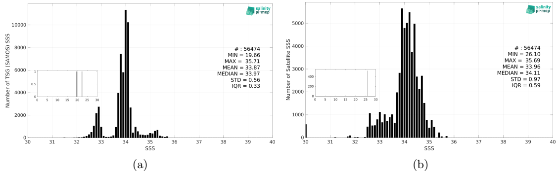
Figure 3: Histograms of SSS from TSG (SAMOS) (a) and Aquarius SSS L3 OR v5 - Monthly - Rain mask (NASA-GSFC) (b) considering all match-up pairs per bins of 0.1 over the Roaring Forties and Furious Fifties Pi-MEP region and for the full satellite product period.
