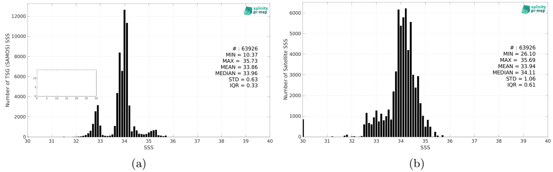
Figure 2: Histograms of SSS from TSG (SAMOS) (a) and Aquarius SSS L3 OR v5 - Monthly - Rain mask (NASA-GSFC) (b) considering all match-up pairs per bins of 0.1 over the Roaring Forties and Furious Fifties Pi-MEP region and for the full satellite product period.
