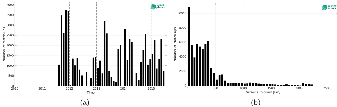
Figure 1: Number of match-ups between TSG (SAMOS) and Aquarius SSS L3 OR v5 - Monthly - Rain mask (NASA-GSFC) SSS as a function of time (a) and as function of the distance to coast (b) over the Roaring Forties and Furious Fifties Pi-MEP region and for the full satellite product period.
