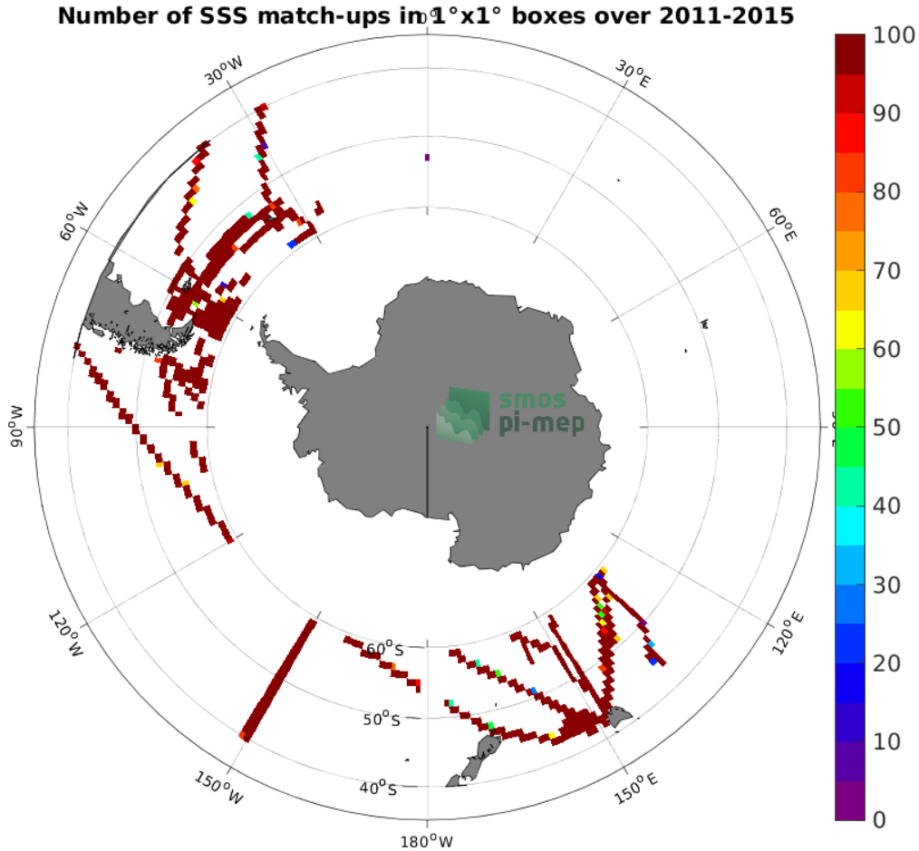
Figure 4: Number of SSS match-ups between TSG (SAMOS) SSS and the Aquarius SSS L3 OR v5 - Monthly - Rain mask (NASA-GSFC) SSS product for the Roaring Forties and Furious Fifties Pi-MEP region over 1^\circ \times 1^\circ boxes and for the full satellite product period.
