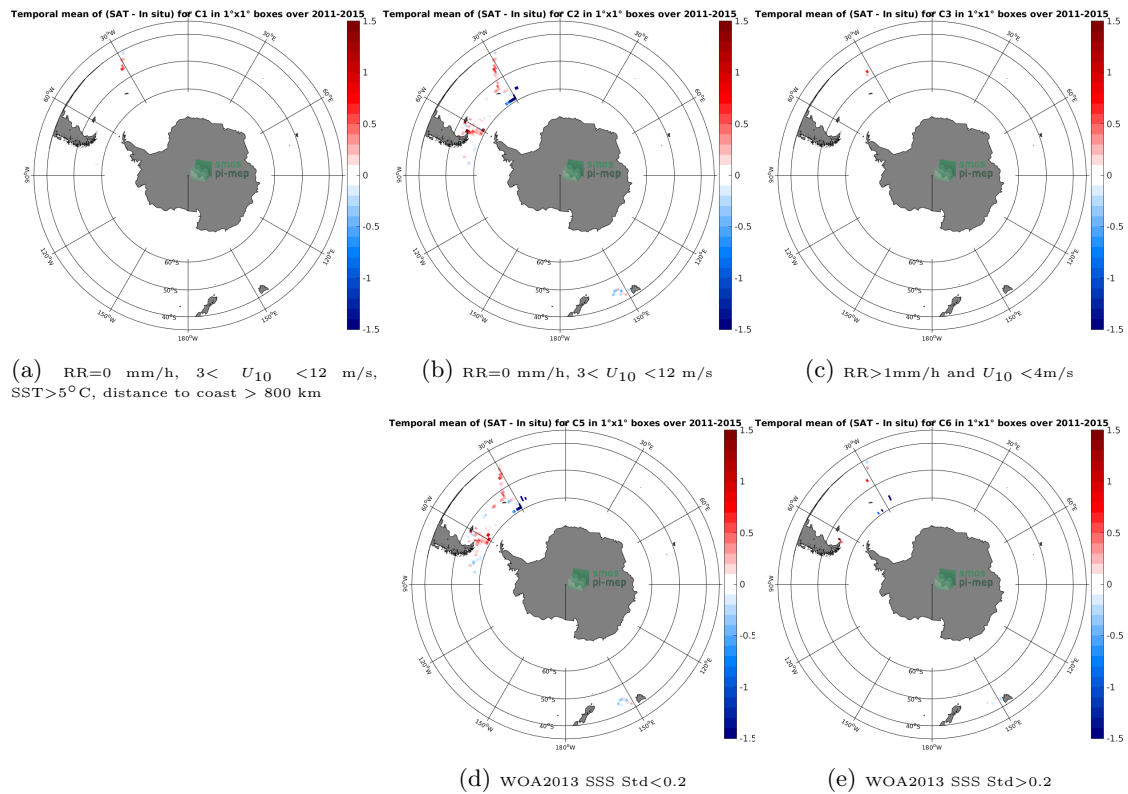
Figure 12: Temporal mean gridded over spatial boxes of size 1^{\circ}\times 1^{\circ} of \Delta\text{SSS} (Aquarius-L3-OR-V5-MONTHLY-RAIN-MASK-1DEG - TSG-SAMOS) for 5 different subdatasets corresponding to:RR=0 mm/h, 3 < U_{10} < 12 m/s, SST >5^{\circ}\text{C} , distance to coast > 800 km (a), RR=0 mm/h, 3 < U_{10} < 12 m/s (b), RR >1 mm/h and U_{10} < 4 m/s (c), WOA2013 SSS Std <0.2 (d), WOA2013 SSS Std >0.2 (e).
