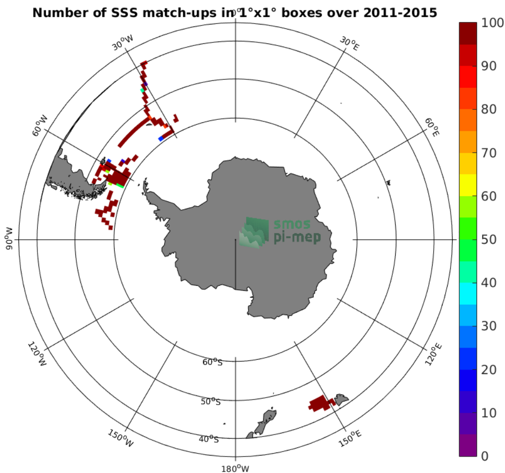
Figure 4: Number of SSS match-ups between TSG-SAMOS SSS and the Aquarius-L3-OR-V5-MONTHLY-RAIN-MASK-1DEG SSS product for the Roaring Forties and Furious Fifties Pi-MEP region over 1°x1° boxes and for the full satellite product period.
