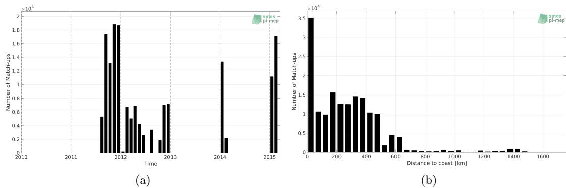
Figure 1: Number of match-ups between TSG-SAMOS and Aquarius-L3-OR-V5-MONTHLY-RAIN-MASK-1DEG SSS as a function of time (a) and as function of the distance to coast (b) over the Roaring Forties and Furious Fifties Pi-MEP region and for the full satellite product period.
