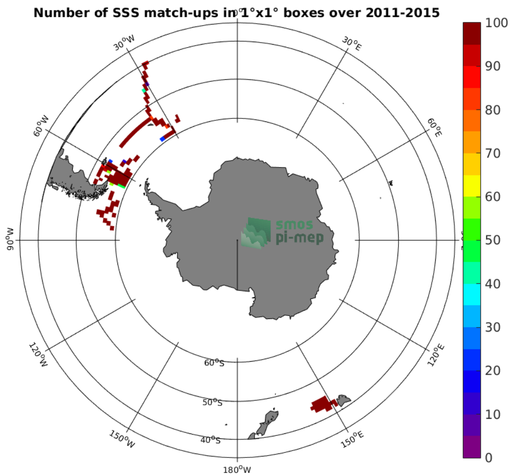
Figure 4: Number of SSS match-ups between TSG-SAMOS SSS and the Aquarius-L3-OR-V5-MONTHLY-RAIN-MASK-1DEG SSS product for the Roaring Forties and Furious Fifties Pi-MEP region over 1^\circ \times 1^\circ boxes and for the full satellite product period.
