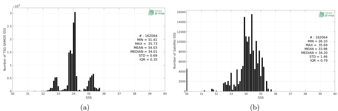
Figure 2: Histograms of SSS from TSG-SAMOS (a) and Aquarius-L3-OR-V5-MONTHLY-RAIN-MASK-1DEG (b) considering all match-up pairs per bins of 0.1 over the Roaring Forties and Furious Fifties Pi-MEP region and for the full satellite product period.
