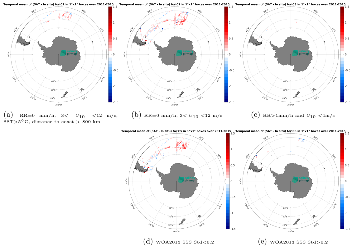
Figure 14: Temporal mean gridded over spatial boxes of size 1^\circ \times 1^\circ of \Delta SSS (Aquarius SSS L3 OR v5 - Monthly - Rain mask (NASA-GSFC) - TSG (Polarstern)) for 5 different subdatasets corresponding to:RR=0 mm/h, 3 < U_{10} < 12 m/s, SST >5^\circ\text{C} , distance to coast > 800 km (a), RR=0 mm/h, 3 < U_{10} < 12 m/s (b), RR >1 mm/h and U_{10} < 4 m/s (c), WOA2013 SSS Std <0.2 (d), WOA2013 SSS Std >0.2 (e).
