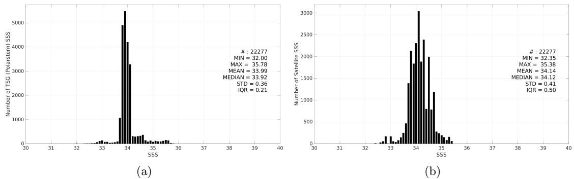
Figure 3: Histograms of SSS from TSG (Polarstern) (a) and Aquarius SSS L3 OR v5 - Monthly - Rain mask (NASA-GSFC) (b) considering all match-up pairs per bins of 0.1 over the Roaring Forties and Furious Fifties Pi-MEP region and for the full satellite product period.
