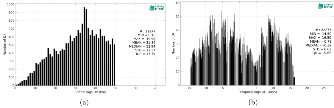
Figure 6: Histograms of the spatial (a) and temporal (b) lags between the location/time of the TSG (Polarstern) measurement and the date of the corresponding Aquarius SSS L3 OR v5 - Monthly - Rain mask (NASA-GSFC) SSS pixel.
