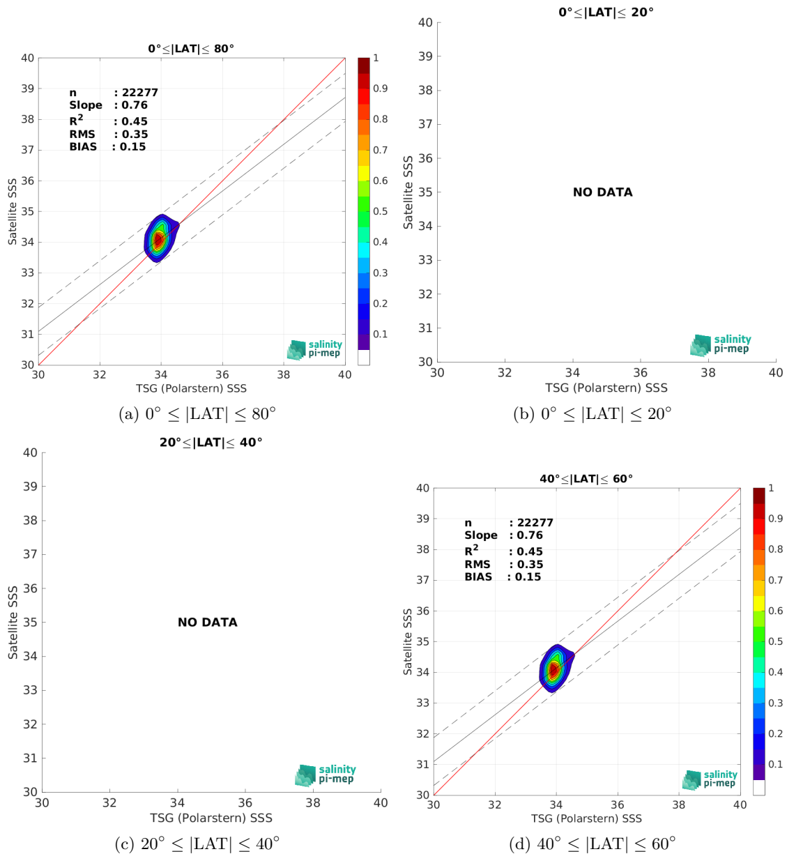
Figure 10: Contour maps of the concentration of Aquarius SSS L3 OR v5 - Monthly - Rain mask (NASA-GSFC) SSS (y-axis) versus TSG (Polarstern) SSS (x-axis) at match-up pairs for different latitude bands. For each plot, the red line shows x=y . The black thin and dashed lines indicate a linear fit through the data cloud and the \pm 95\% confidence levels, respectively. The number match-up pairs n , the slope and R^2 coefficient of the linear fit, the root mean square (RMS) and the mean bias between satellite and in situ data are indicated for each latitude band in each plots.
