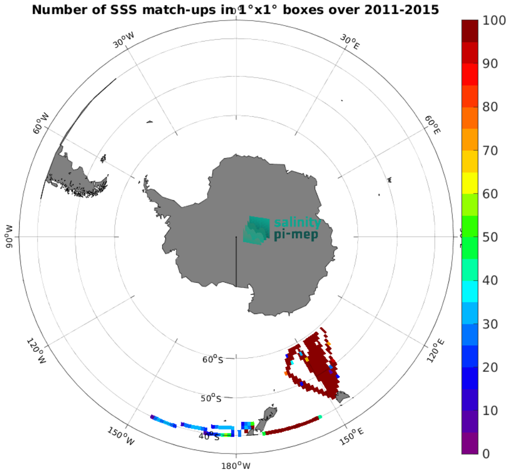
Figure 5: Number of SSS match-ups between TSG (LEGOS-DM) SSS and the Aquarius SSS L3 OR v5 - Monthly - Rain mask (NASA-GSFC) SSS product for the Roaring Forties and Furious Fifties Pi-MEP region over 1^\circ \times 1^\circ boxes and for the full satellite product period.
