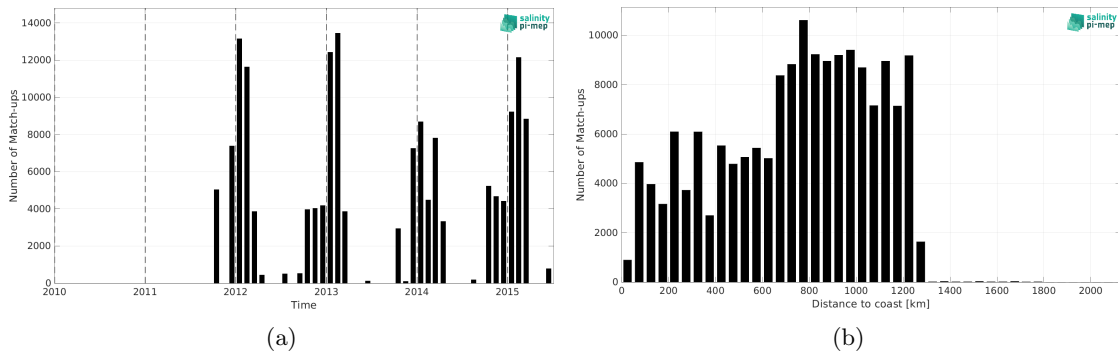
Figure 2: Number of match-ups between TSG (LEGOS-DM) and Aquarius SSS L3 OR v5 - Monthly - Rain mask (NASA-GSFC) SSS as a function of time (a) and as function of the distance to coast (b) over the Roaring Forties and Furious Fifties Pi-MEP region and for the full satellite product period.
