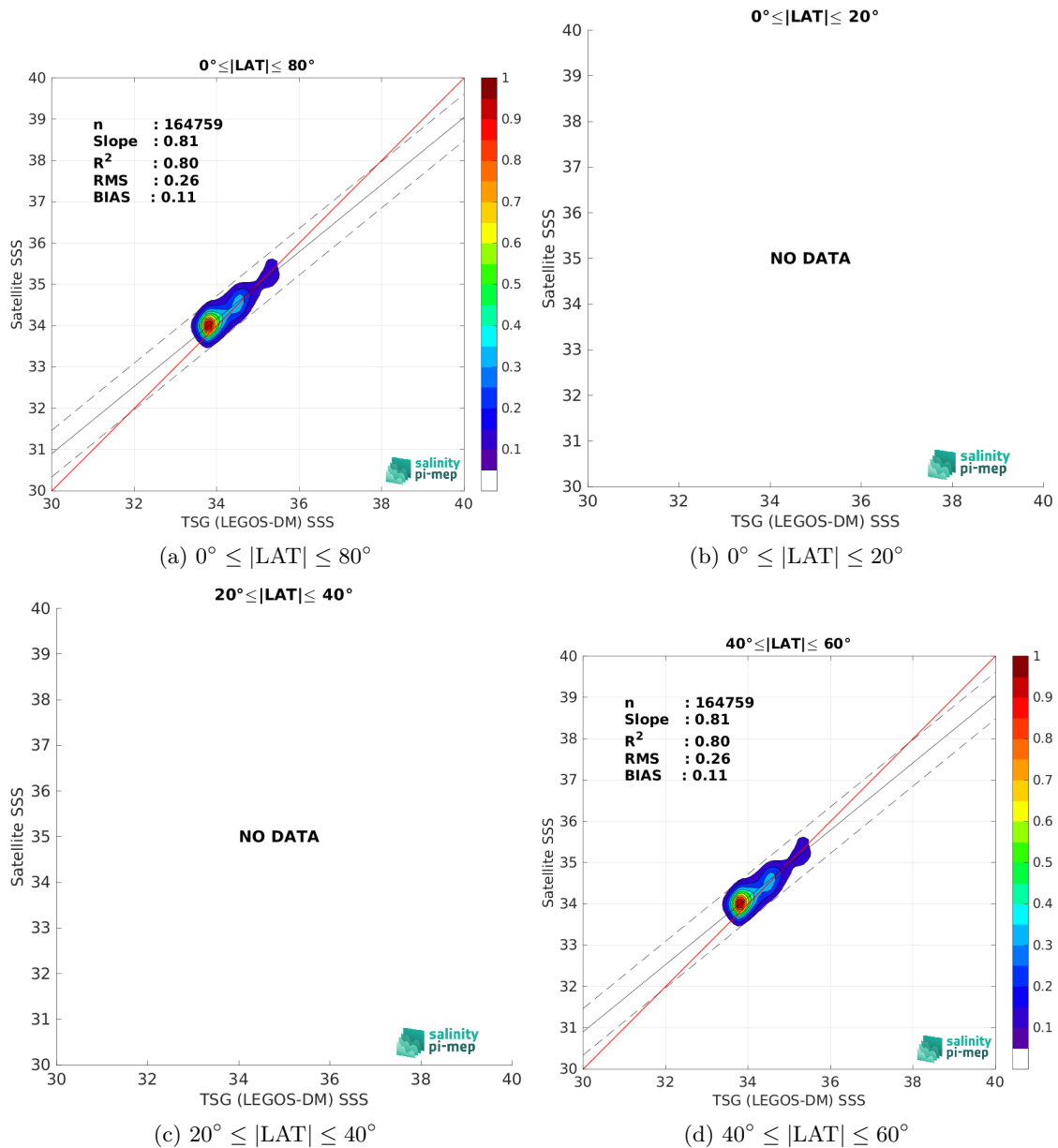
Figure 10: Contour maps of the concentration of Aquarius SSS L3 OR v5 - Monthly - Rain mask (NASA-GSFC) SSS (y-axis) versus TSG (LEGOS-DM) SSS (x-axis) at match-up pairs for different latitude bands. For each plot, the red line shows x=y . The black thin and dashed lines indicate a linear fit through the data cloud and the \pm 95\% confidence levels, respectively. The number match-up pairs n , the slope and R^2 coefficient of the linear fit, the root mean square (RMS) and the mean bias between satellite and in situ data are indicated for each latitude band in each plots.
