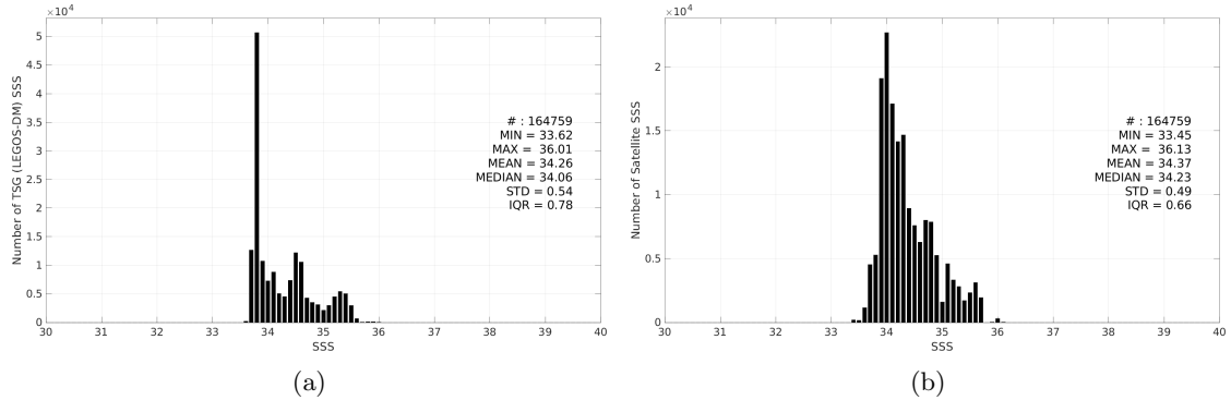
Figure 3: Histograms of SSS from TSG (LEGOS-DM) (a) and Aquarius SSS L3 OR v5 - Monthly - Rain mask (NASA-GSFC) (b) considering all match-up pairs per bins of 0.1 over the Roaring Forties and Furious Fifties Pi-MEP region and for the full satellite product period.
