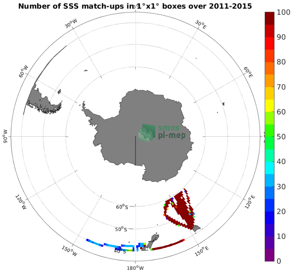
Figure 4: Number of SSS match-ups between TSG (LEGOS-DM) SSS and the Aquarius SSS L3 OR v5 - Monthly - Rain mask (NASA-GSFC) SSS product for the Roaring Forties and Furious Fifties Pi-MEP region over 1^\circ \times 1^\circ boxes and for the full satellite product period.
