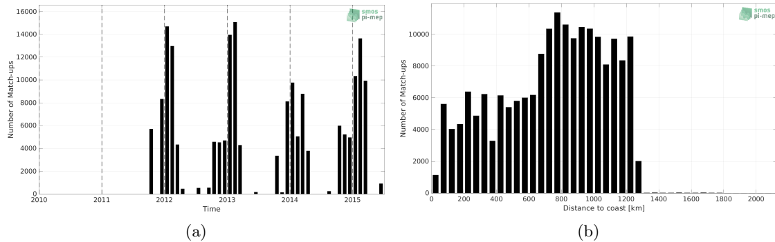
Figure 1: Number of match-ups between TSG (LEGOS-DM) and Aquarius SSS L3 OR v5 - Monthly - Rain mask (NASA-GSFC) SSS as a function of time (a) and as function of the distance to coast (b) over the Roaring Forties and Furious Fifties Pi-MEP region and for the full satellite product period.
