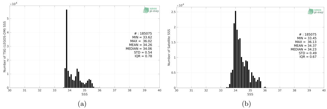
Figure 2: Histograms of SSS from TSG (LEGOS-DM) (a) and Aquarius SSS L3 OR v5 - Monthly - Rain mask (NASA-GSFC) (b) considering all match-up pairs per bins of 0.1 over the Roaring Forties and Furious Fifties Pi-MEP region and for the full satellite product period.
