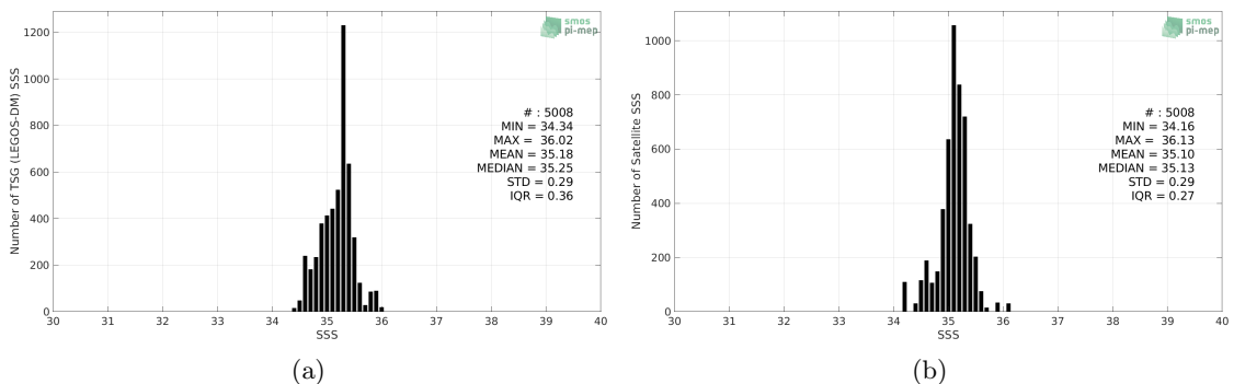
Figure 2: Histograms of SSS from TSG (LEGOS-DM) (a) and Aquarius SSS L3 OR v5 - Monthly - Rain mask (NASA-GSFC) (b) considering all match-up pairs per bins of 0.1 over the Roaring Forties and Furious Fifties Pi-MEP region and for the full satellite product period.
