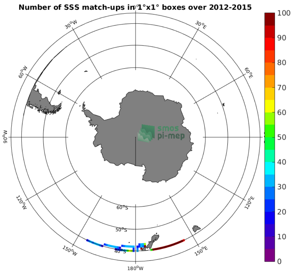
Figure 4: Number of SSS match-ups between TSG-LEGOS-DM SSS and the Aquarius-L3-OR-V5-MONTHLY-RAIN-MASK-1DEG SSS product for the Roaring Forties and Furious Fifties Pi-MEP region over 1°x1° boxes and for the full satellite product period.
