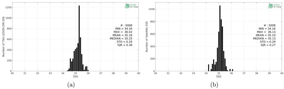
Figure 2: Histograms of SSS from TSG-LEGOS-DM (a) and Aquarius-L3-OR-V5-MONTHLY-RAIN-MASK-1DEG (b) considering all match-up pairs per bins of 0.1 over the Roaring Forties and Furious Fifties Pi-MEP region and for the full satellite product period.
