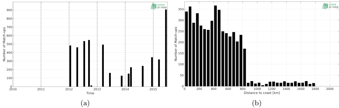
Figure 1: Number of match-ups between TSG-LEGOS-DM and Aquarius-L3-OR-V5-MONTHLY-RAIN-MASK-1DEG SSS as a function of time (a) and as function of the distance to coast (b) over the Roaring Forties and Furious Fifties Pi-MEP region and for the full satellite product period.
