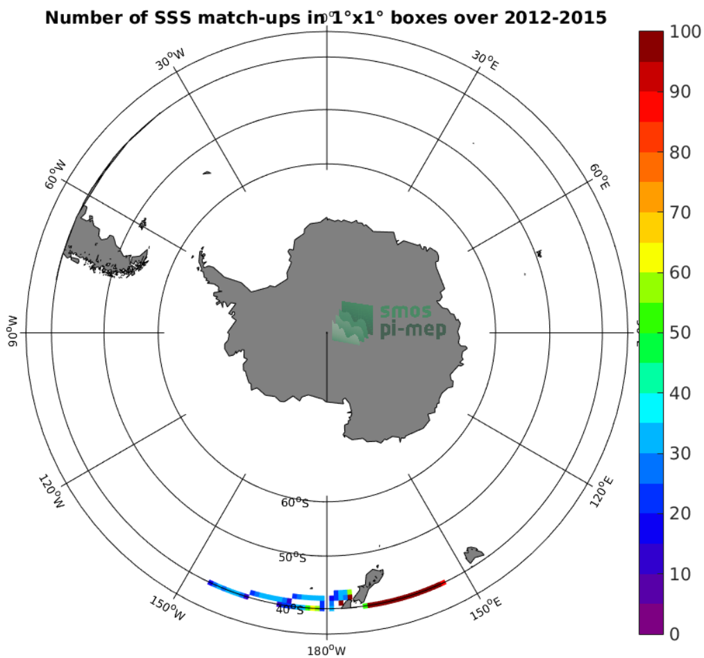
Figure 4: Number of SSS match-ups between TSG-LEGOS-DM SSS and the Aquarius-L3-OR-V5-MONTHLY-RAIN-MASK-1DEG SSS product for the Roaring Forties and Furious Fifties Pi-MEP region over 1^\circ \times 1^\circ boxes and for the full satellite product period.
