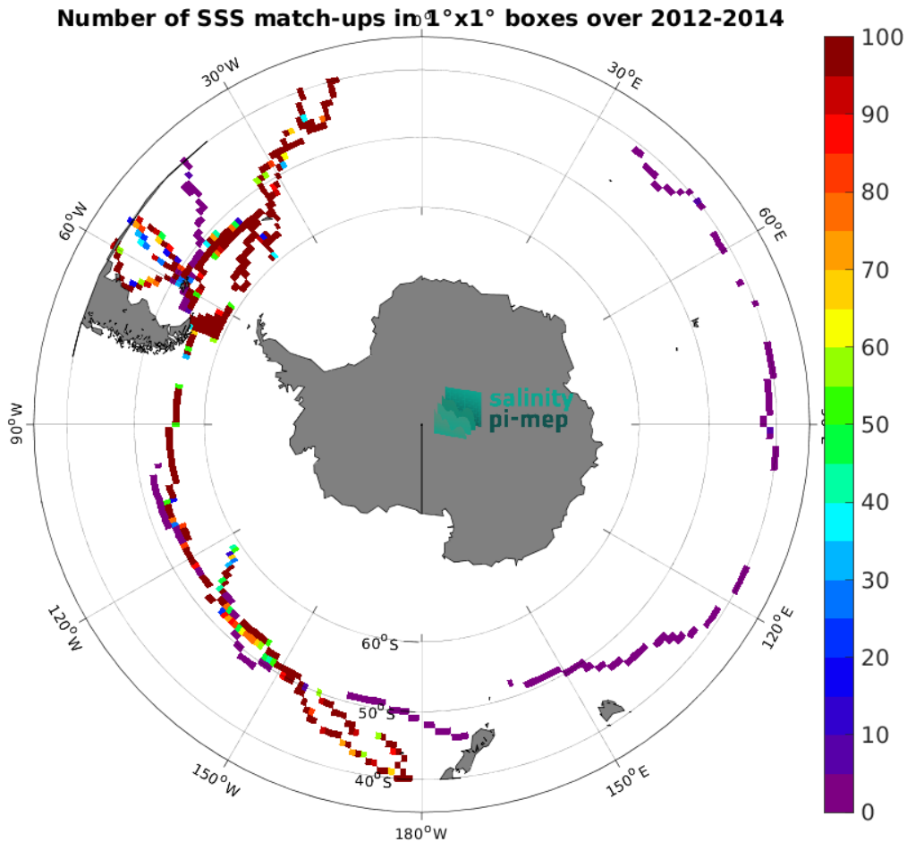
Figure 5: Number of SSS match-ups between TSG (GOSUD-Sailing-ship) SSS and the Aquarius SSS L3 OR v5 - Monthly - Rain mask (NASA-GSFC) SSS product for the Roaring Forties and Furious Fifties Pi-MEP region over 1^\circ \times 1^\circ boxes and for the full satellite product period.
