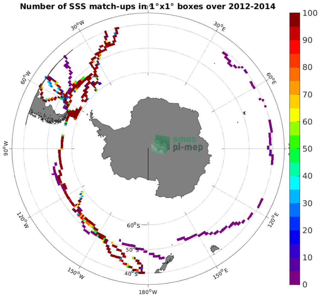
Figure 4: Number of SSS match-ups between TSG (GOSUD-Sailing-ship) SSS and the Aquarius SSS L3 OR v5 - Monthly - Rain mask (NASA-GSFC) SSS product for the Roaring Forties and Furious Fifties Pi-MEP region over 1^\circ \times 1^\circ boxes and for the full satellite product period.
