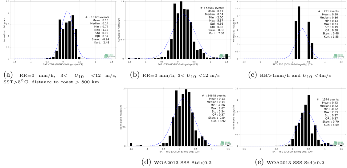
Figure 13: Normalized histogram of \Delta\text{SSS} (Aquarius SSS L3 OR v5 - Monthly - Rain mask (NASA-GSFC) - TSG (GOSUD-Sailing-ship)) for 5 different subdatasets corresponding to: RR=0 mm/h, 3 < U_{10} < 12 m/s, SST>5°C, distance to coast > 800 km (a), RR=0 mm/h, 3 < U_{10} < 12 m/s (b), RR>1mm/h and U_{10} < 4 m/s (c), WOA2013 SSS Std<0.2 (d), WOA2013 SSS Std>0.2 (e).
