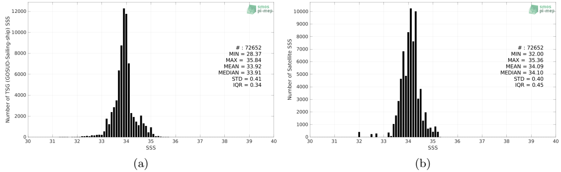
Figure 2: Histograms of SSS from TSG (GOSUD-Sailing-ship) (a) and Aquarius SSS L3 OR v5 - Monthly - Rain mask (NASA-GSFC) (b) considering all match-up pairs per bins of 0.1 over the Roaring Forties and Furious Fifties Pi-MEP region and for the full satellite product period.
