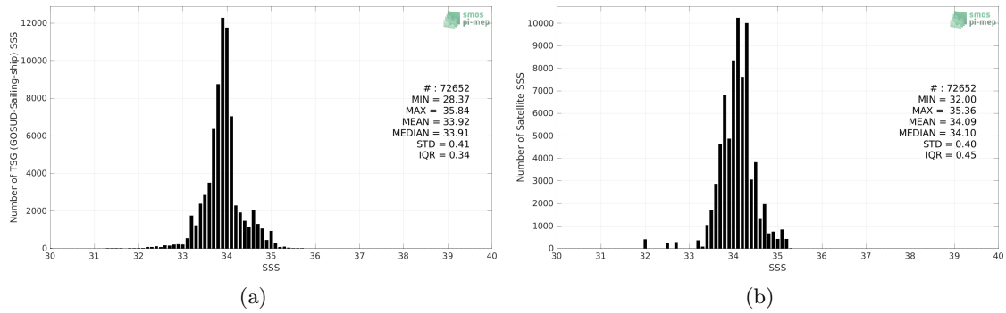
Figure 2: Histograms of SSS from TSG (GOSUD-Sailing-ship) (a) and Aquarius SSS L3 OR v5 - Monthly - Rain mask (NASA-GSFC) (b) considering all match-up pairs per bins of 0.1 over the Roaring Forties and Furious Fifties Pi-MEP region and for the full satellite product period.
