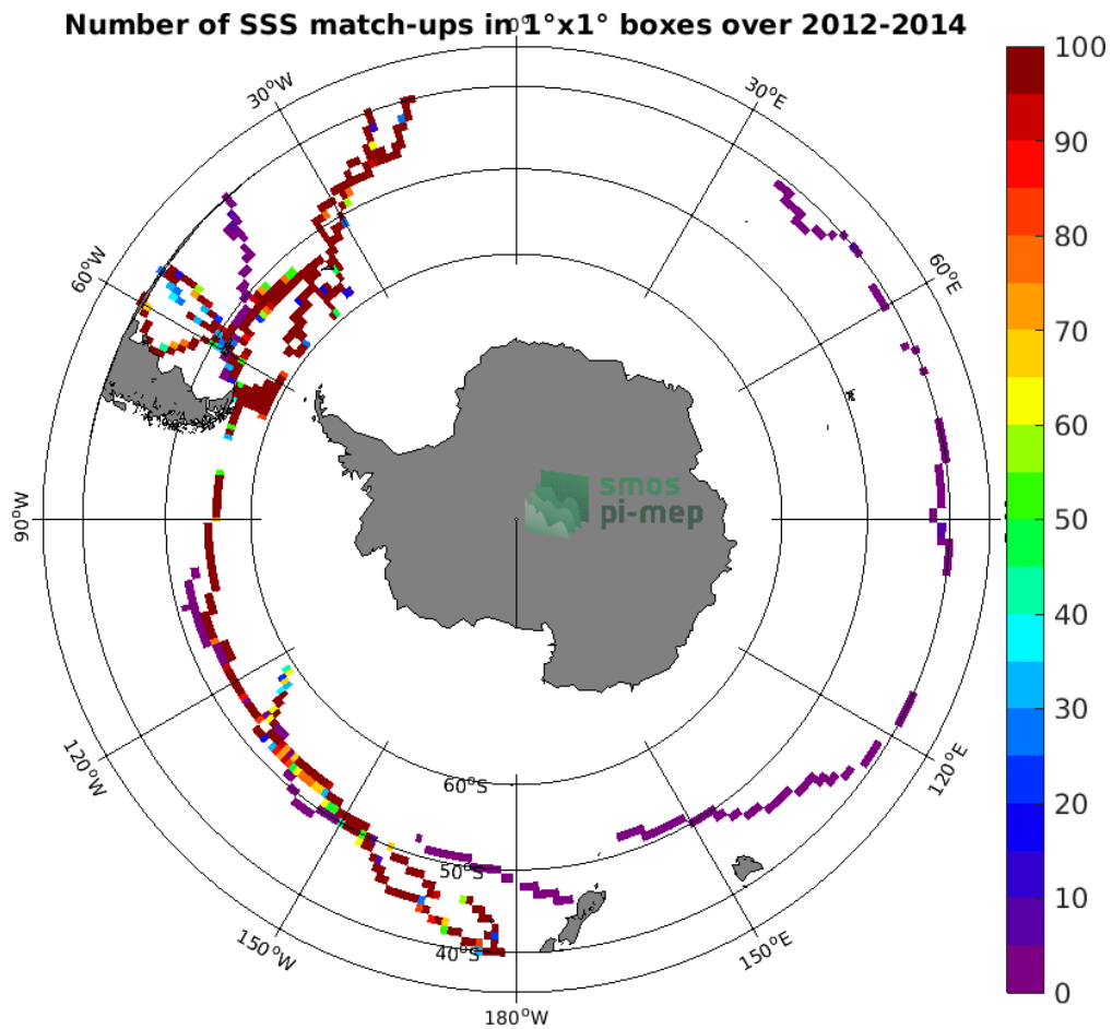
Figure 4: Number of SSS match-ups between TSG (GOSUD-Sailing-ship) SSS and the Aquarius SSS L3 OR v5 - Monthly - Rain mask (NASA-GSFC) SSS product for the Roaring Forties and Furious Fifties Pi-MEP region over 1^\circ \times 1^\circ boxes and for the full satellite product period.
