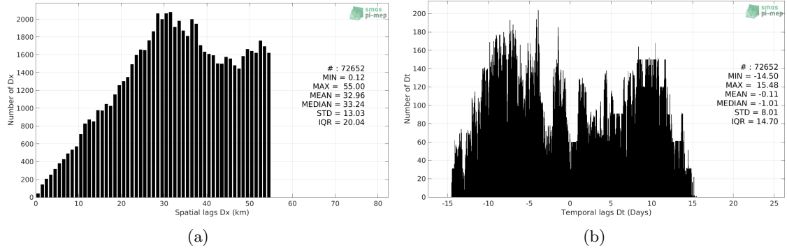
Figure 5: Histograms of the spatial (a) and temporal (b) lags between the time of the TSG (GOSUD-Sailing-ship) measurements and the date of the corresponding Aquarius SSS L3 OR v5 - Monthly - Rain mask (NASA-GSFC) SSS product.
